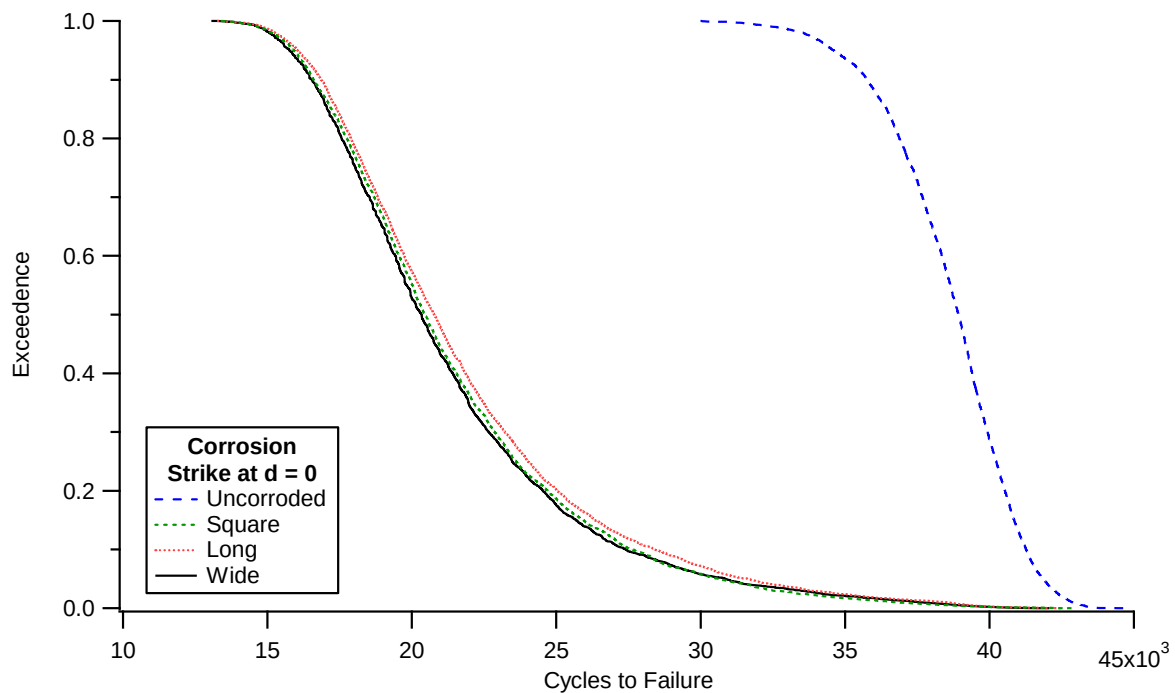
Figure 60: Effect of Wide, Long and Square corrosion strikes centred at d = 0 (specimen midpoint) on fatigue life compared to predicted fatigue life of an uncorroded specimen
