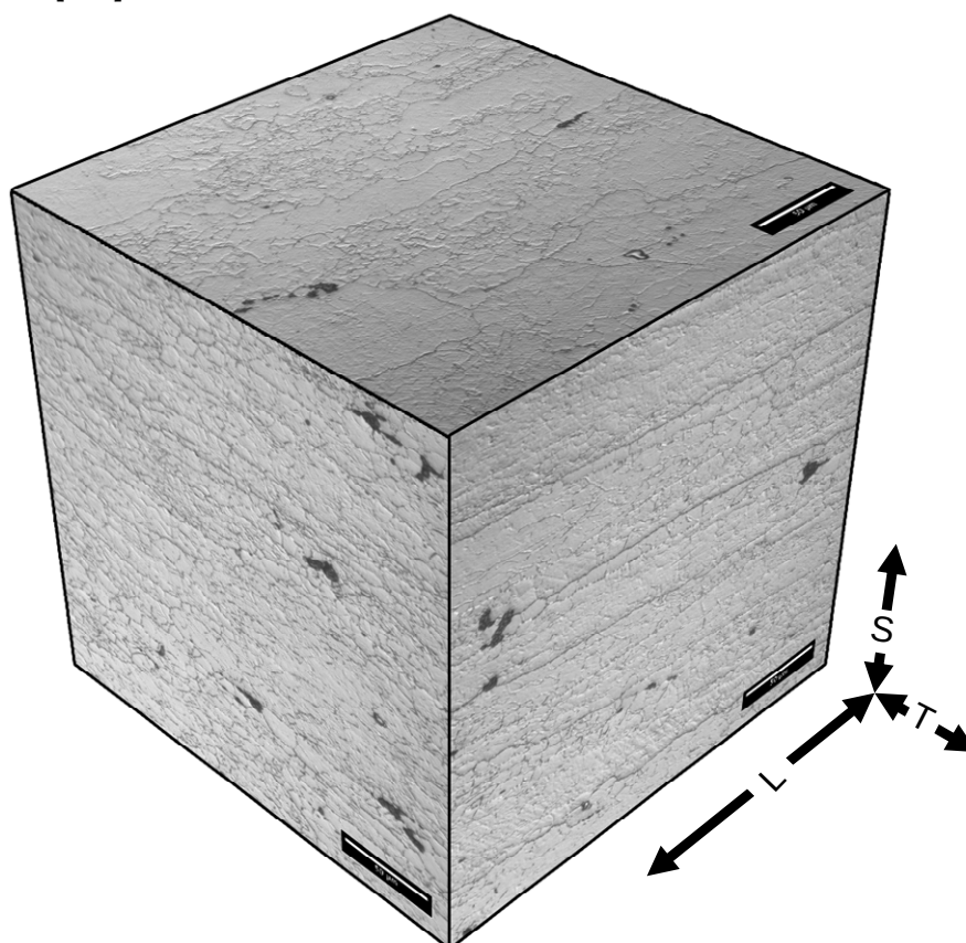
Figure 9: Three-plane micrograph of etched 7010-T7651 showing the grain boundaries and inclusions. Scale bars indicate 50 \mu\text{m} .
