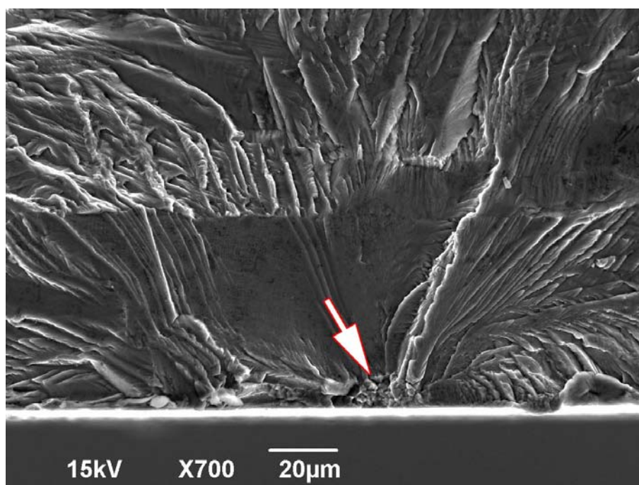
Figure 73: SEM micrographs of (a) Specimen 24E showing the corrosion pit, highlighted in red, from which fatigue cracks have initiated on two levels and (b) the crack initiating particle on Specimen B3. Note that the particle (indicated by a white arrow) is far smaller than the corrosion pit in part (a).
