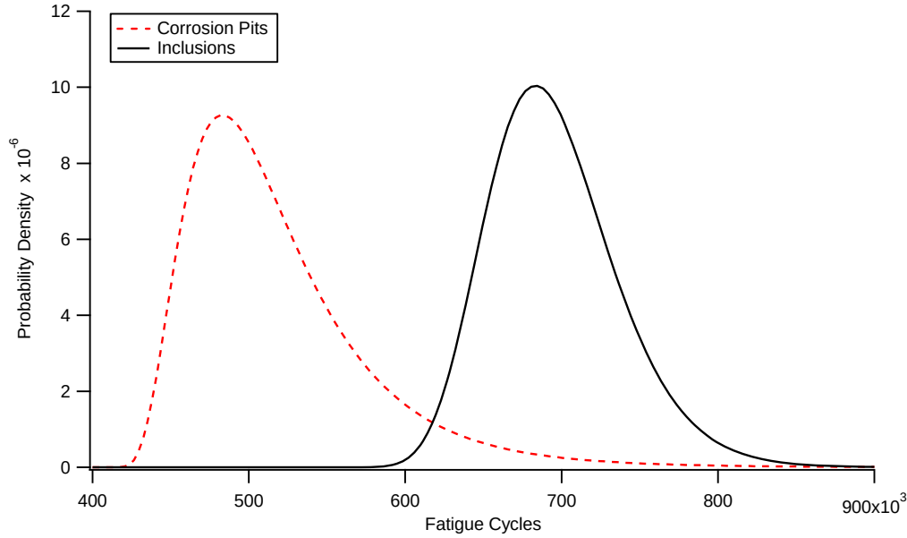
Figure 74: Plot of the PDFs of the predicted fatigue life distributions for corrosion pits and inclusions.
