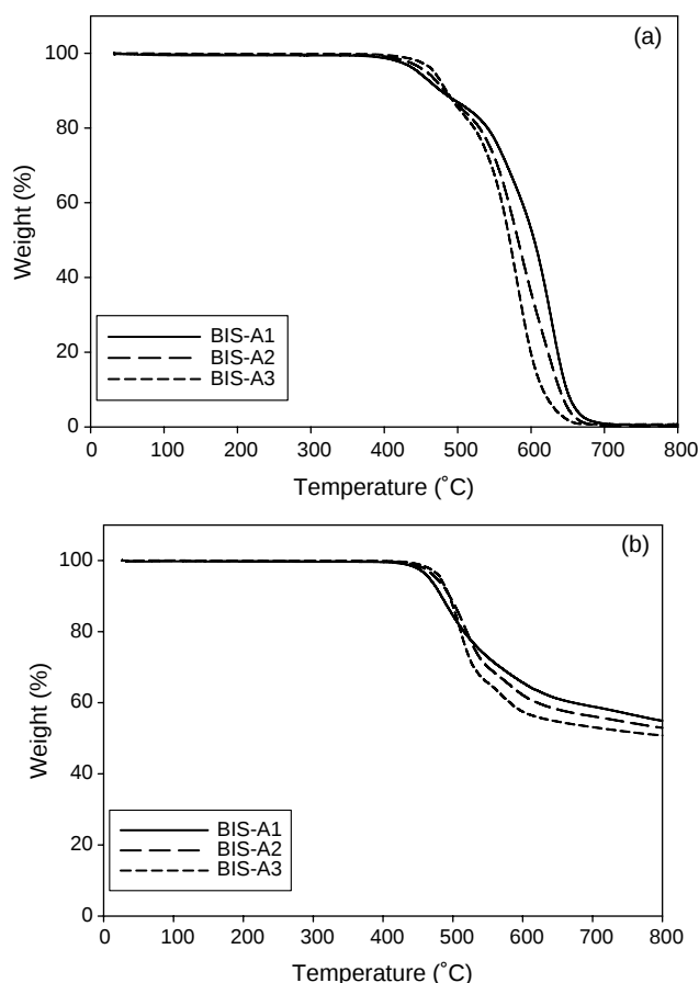
Fig. 7. TGA thermograms of BIS-A1-3 after having being cured at 300 °C for 30 min and 350 °C for 30 min (a) in air; (b) in nitrogen.
