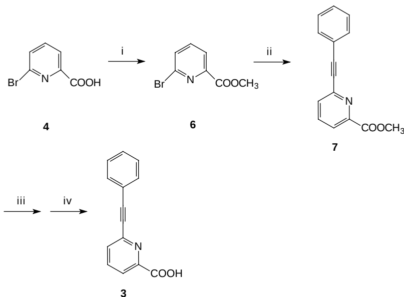
Scheme 3. Chemical synthesis of 6-phenylethynyl picolinic acid (i) methyl iodide, DBU, acetonitrile, 12 h; (ii) phenylacetylene, \text{PdCl}_2(\text{PPh}_3)_2 , CuI, \text{PPh}_3 , \text{NEt}_3 , reflux, 4 h; (iii) \text{Na}_2\text{CO}_3 , MeOH, Reflux, 4 h; (iv) acetic acid.
