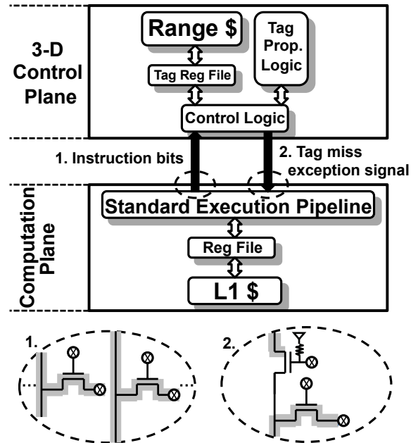
Fig. 14. A 3D system monitor tracking data flow on the computation plane. This is achieved by Tapping (1) the instructions that we want to track and Overriding (2) to raise an exception signal.
