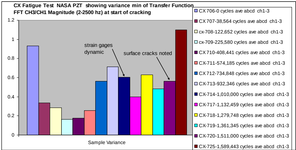
Figure 5 CX-100 FRF transmissibility (averaged areas) of the PZT system for sensor1 to sensor3
