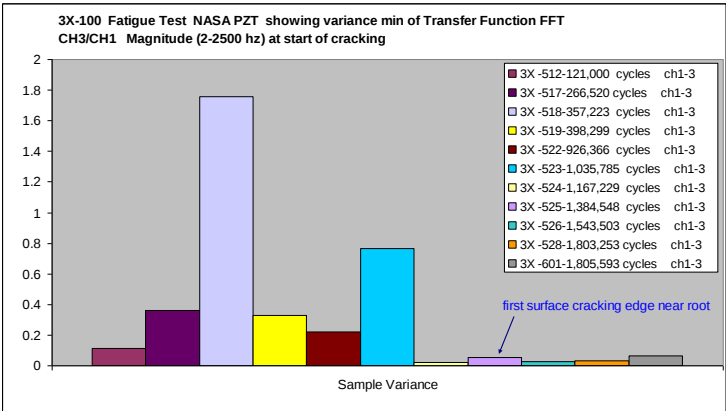
Figure 4 shows the TX-100 FRF transmissibility (averaged variances) of the PZT system for sensor 1
