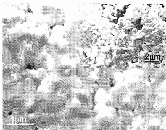
Figure 1 SEM micrograph of biosilica-immobilized butyrylcholinesterase.
