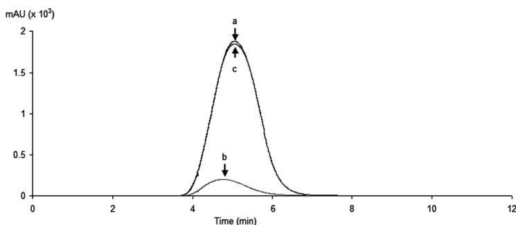
Figure 3. Screening of a cholinesterase inhibitor on a BuChE-IMER. Chromatograms showing subsequent injections to a BuChE-IMER of butyrylthiocholine at saturating substrate concentration (a), with 1 mM tacrine inhibitor (b), and again with butyrylthiocholine at saturating substrate concentration (c).
