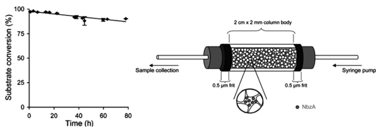
Figure 5. Silica-immobilized nitroreductase IMER. Schematic of the IMER containing silica-encapsulated nitroreductase inside a stainless steel microreactor (specifications shown) and operational stability of the resulting column for the conversion of nitrobenzene (100 \mu M) at 5 \mu L/min. Source: Figures reprinted with permission from Biomacromolecules , 2006, 7, 2631–2636. [87] Copyright 2006 American Chemical Society.
