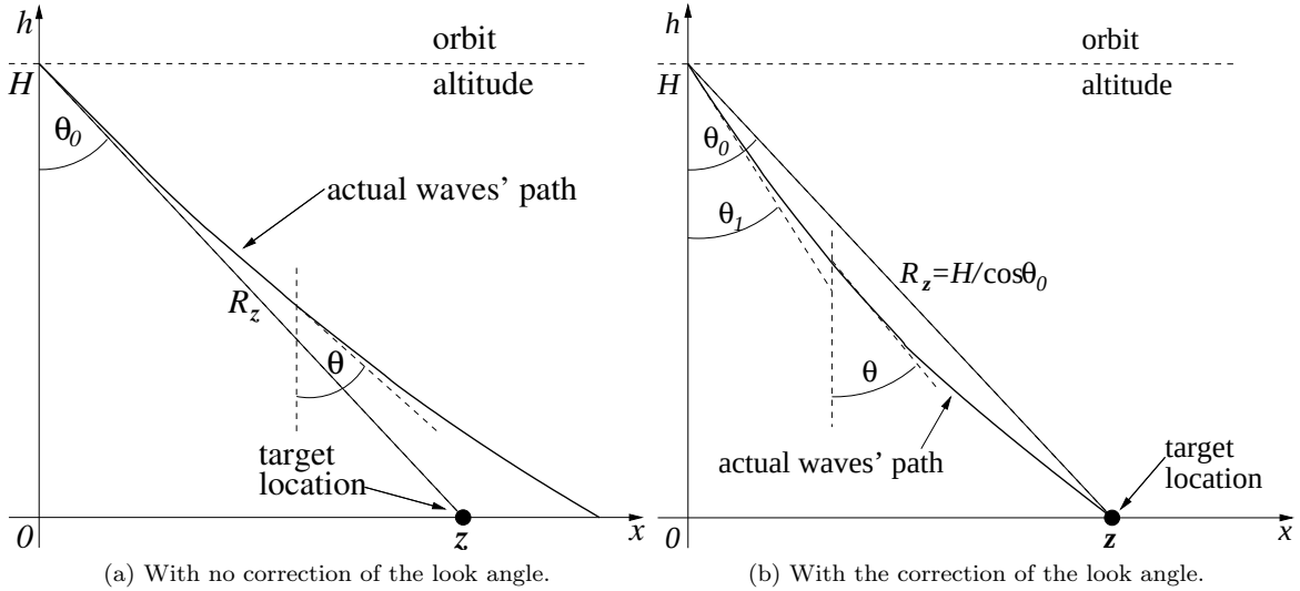
Figure C.1: Schematic waves' travel paths between the antenna and the target in the inhomogeneous ionosphere.
