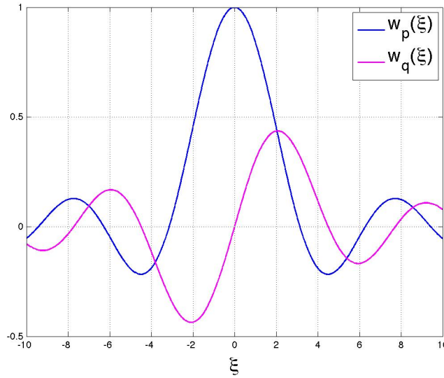
Figure 3.1: Components of the range factor (3.19) in the presence of the Faraday rotation.
