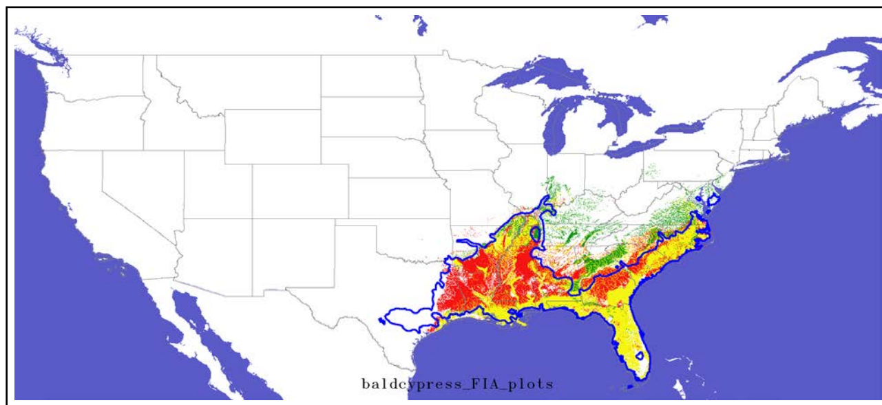
Figure 11. Climate affects on Bald Cypress ( Taxodium distichum ).
