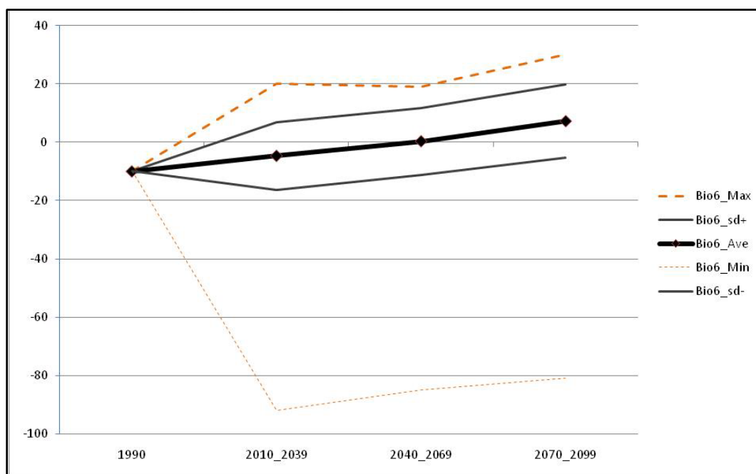
Figure 4. Minimum temperature of coldest month ( ^{\circ}\text{C} \times 10 ): average, SD, maximum, minimum all GCMs and scenarios.
