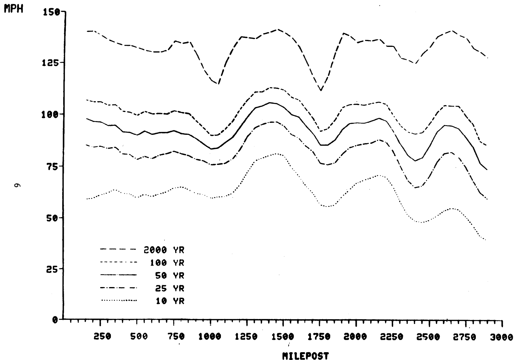
Figure 2. Estimated fastest-mile hurricane wind speeds blowing from any direction at 10 m above ground in open terrain near the coastline, for various mean recurrence intervals (1 mph = 0.47 m/s). (Battes, et. al., 1980)
