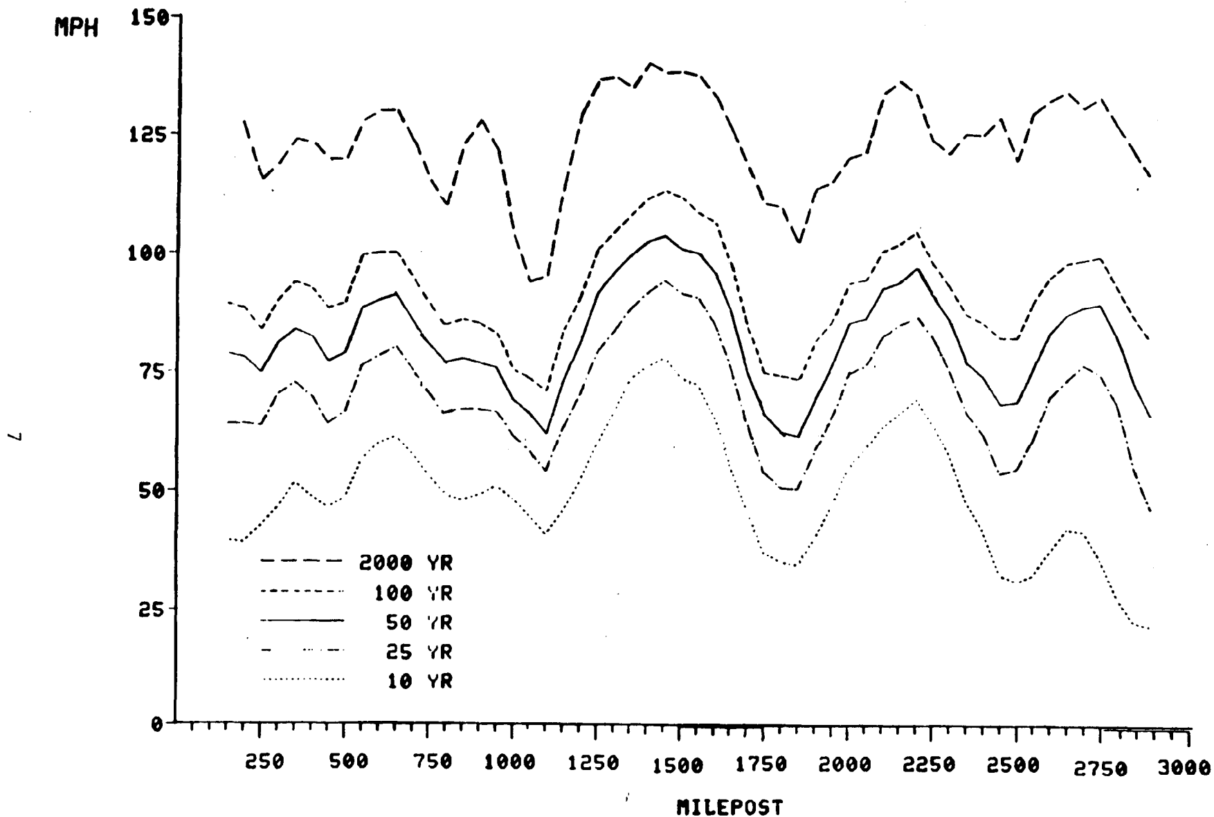
Figure 3. Estimated fastest-mile hurricane wind speeds blowing from any direction at 10 m above ground in open terrain at 200 km inland, for various mean recurrence intervals (1 mph = 0.47 m/s). (Batts, et. al., 1980)
