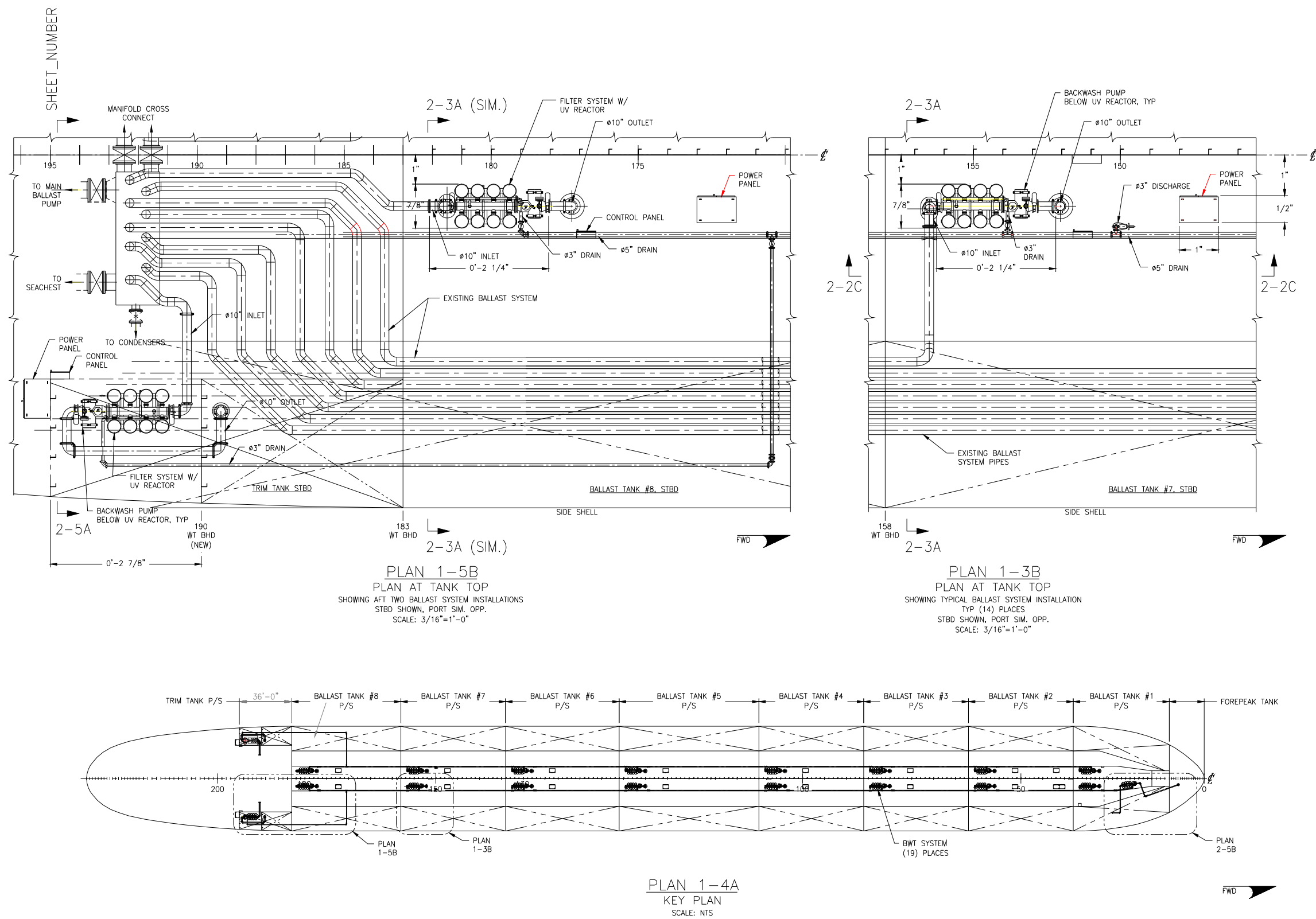
Figure C-1. Vessel Three, BWT System 1 (filter/UV BWT System): general arrangement (1 of 2).
