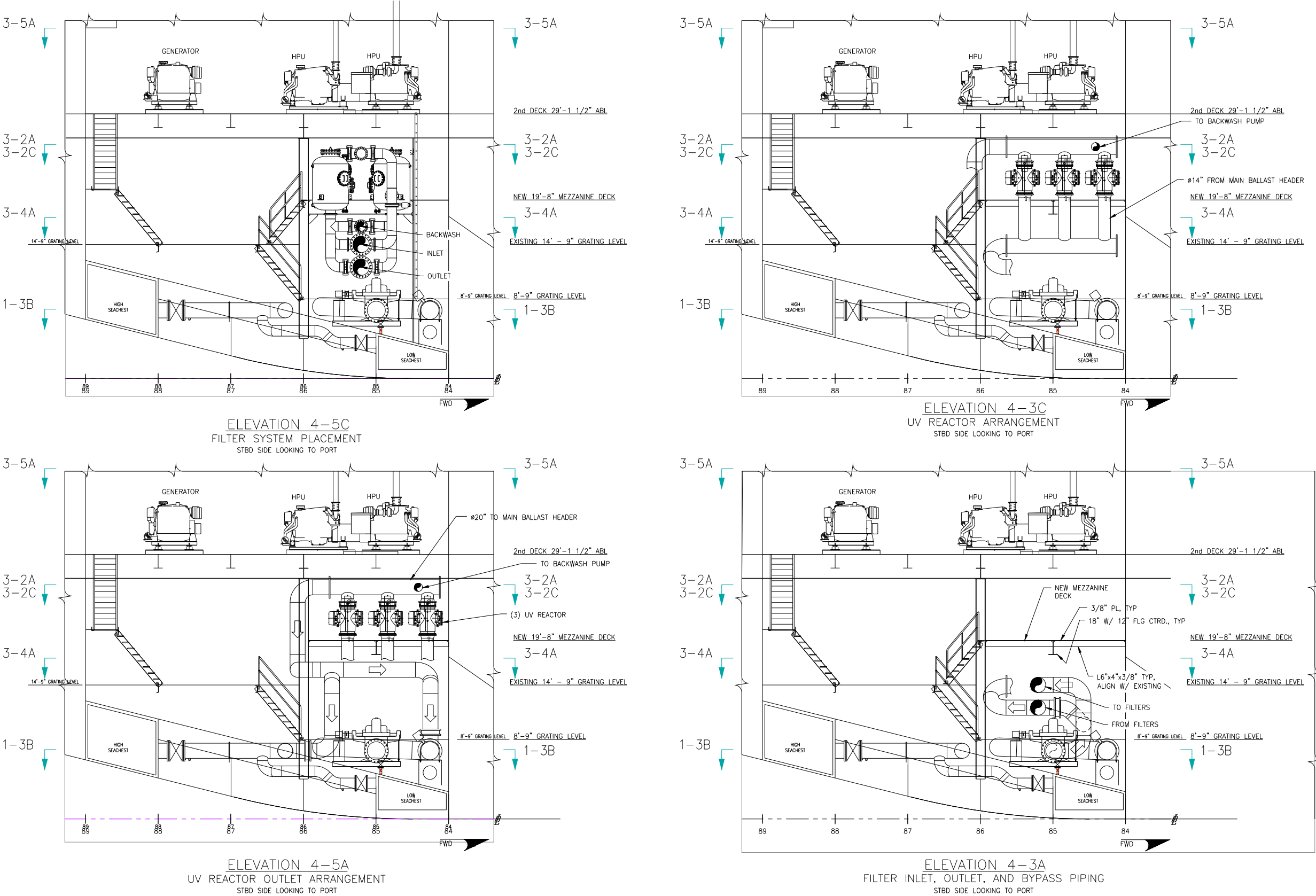
Figure D-1. Vessel Four, BWT System 1 (filter/UV BWT): general arrangement (4 of 4).
