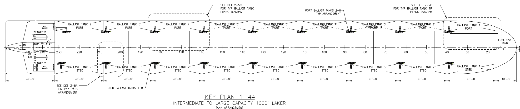
Figure A-1. Vessel One, BWT System 1 (filter/UV BWT System): piping diagram and general arrangement (1 of 3).
