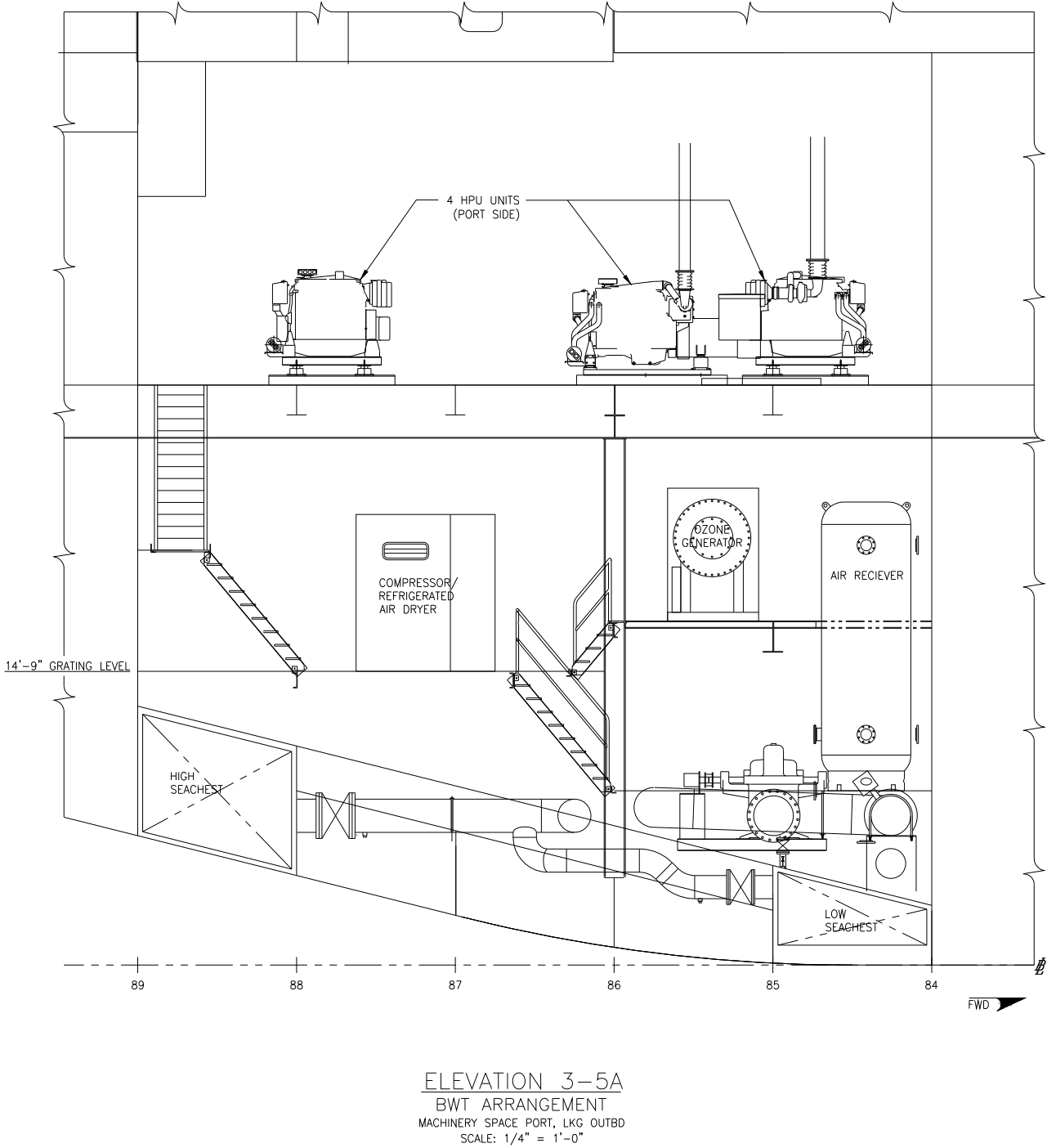
Figure D-3. Vessel Four, BWT System 2 (ozone BWT System): general arrangement (3 of 3).
