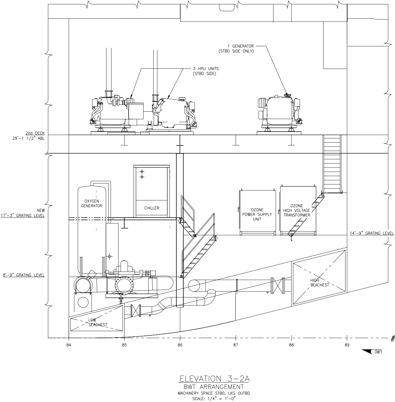
Figure D-3. Vessel Four, BWT System 2 (ozone BWT System): general arrangement (3 of 3).
