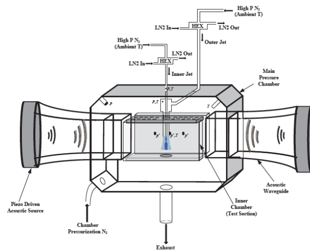
Figure 1 Schematic of experimental chamber and fluid systems
