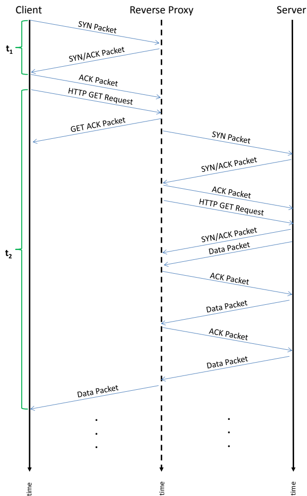
Figure 3.6: Reverse Proxy Connection RTTs
