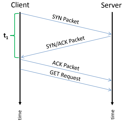
Figure 4.1: Packet Timing Diagram for Failed GET Requests
