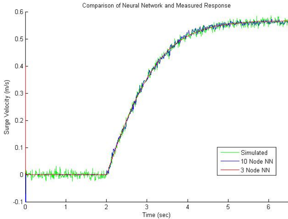
Figure 21. Comparison of actual surge velocities to 10 node and three node NARX
