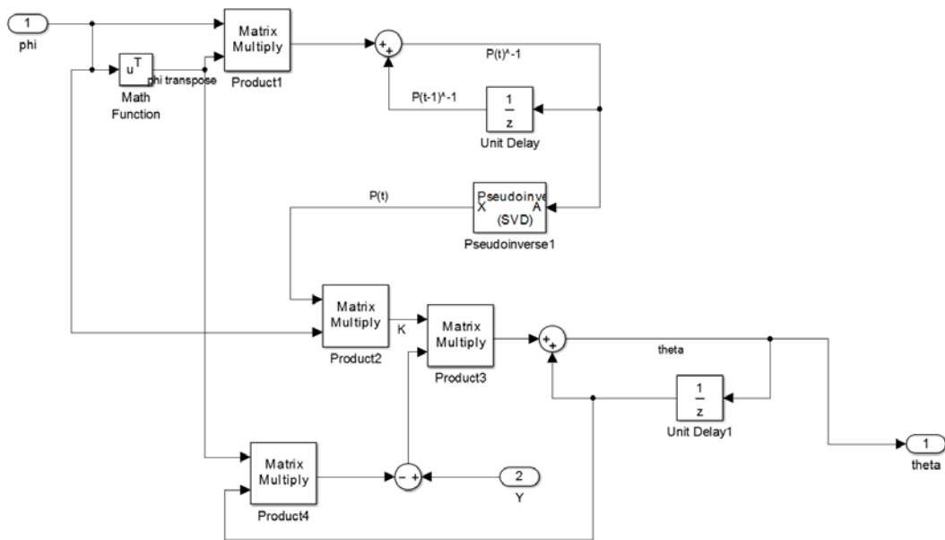
Figure 28. RLS estimator
