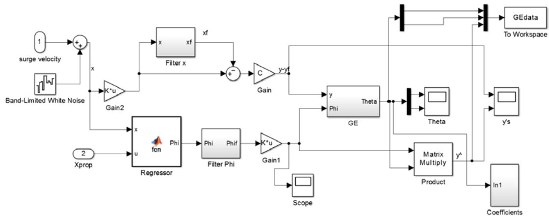
Figure 29. Gradient estimator
