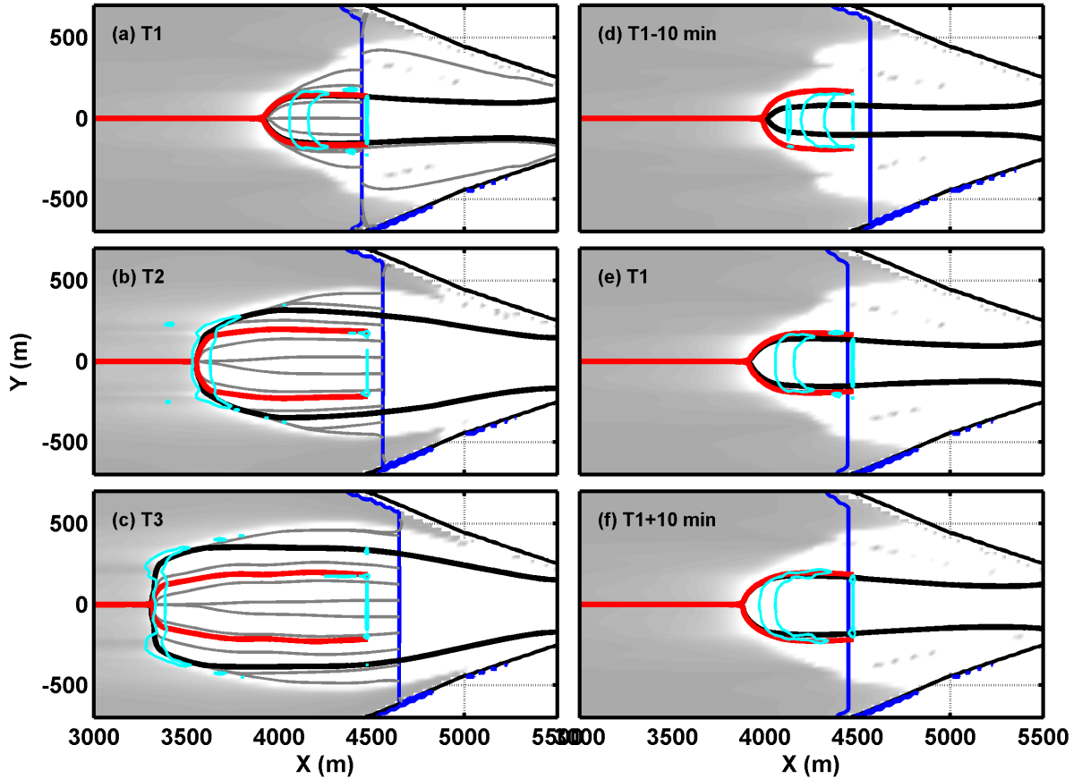
Figure 12. Information flow plots in the baseline bathymetry at the analyzed time steps (a-c) and individual time steps near the flood transition (d-f) . Black lines are expansion envelopes, and outline the region that is uninformed about the basin expansion. Red lines show the slope break envelope, and encompass the region containing slope break information. Gray lines are drawn from the calculated plunge section (drawn in blue) and indicate where the flow
