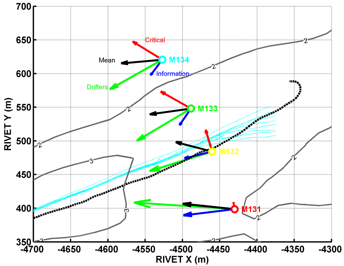
Figure 22. Mean velocity vectors (subsurface ADCP and surface drifters ) and rotated components ( critical and information ). Dashed black line shows the GPS track of the visual small boat trace of the front on 09 May. Cyan lines show the drifter traces from the deployment set closest to the observed front on 13 May. Gray contours are labeled in meters.
