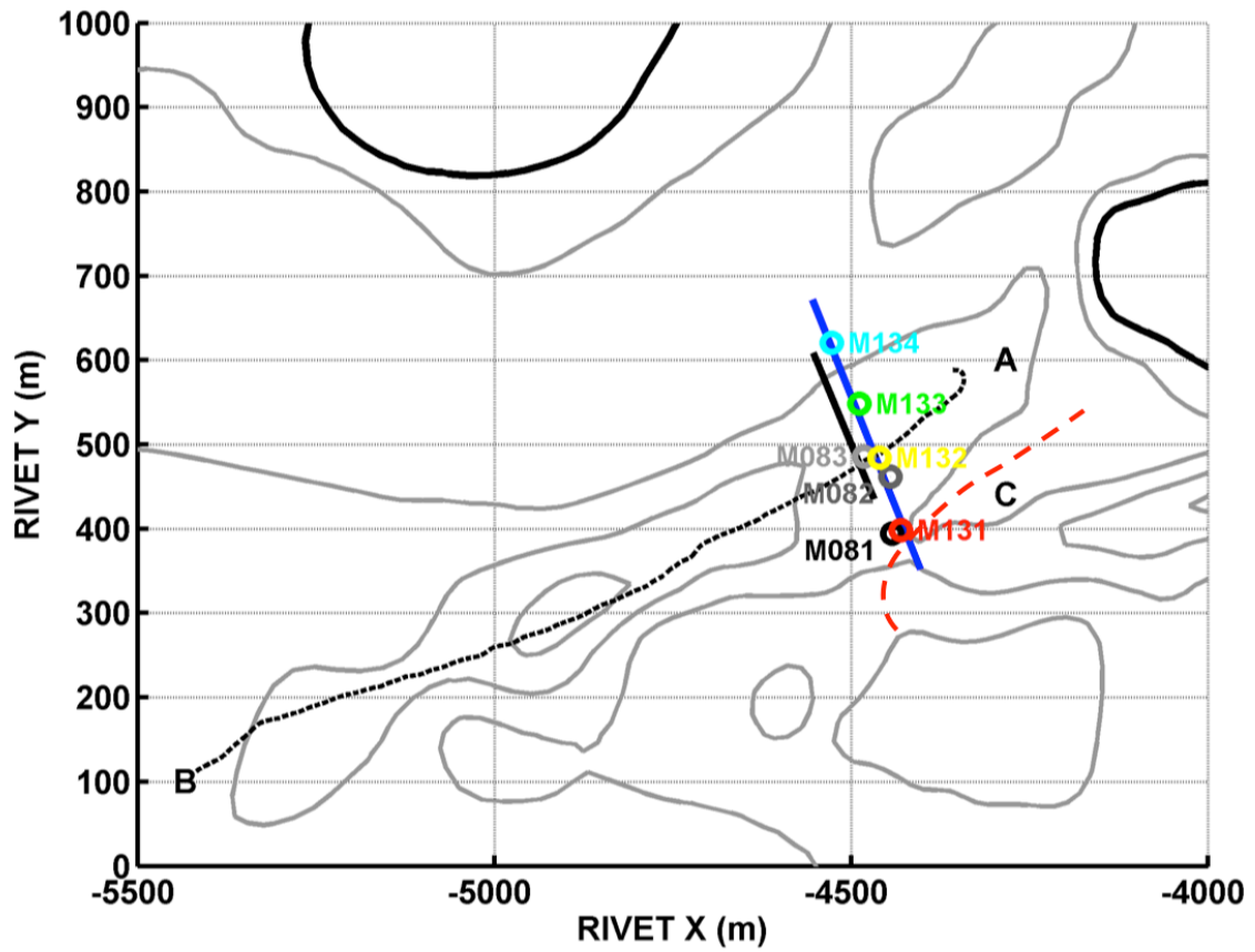
Figure 15. Mini-cats (●), transects (lines), and GPS surface front trace (dashed black line A-B) discussed in this paper. Front trace and blue transect line match those shown in Figure 14. Black and gray mini-cat locations were collected 08-09 May; colored locations on 13 May 2012. The red dashed curve marks the location of the sill at the intersection of the main tidal channel and the secondary channel that induces the front. Contours are 1 meter depth intervals.
