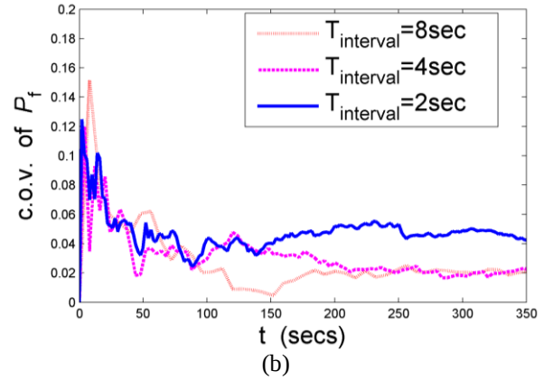
Figure 9. C.O.V. of failure rate (a) and probability of failure (b) from SS/SPT method for 2, 4, and 8 sec intervals
