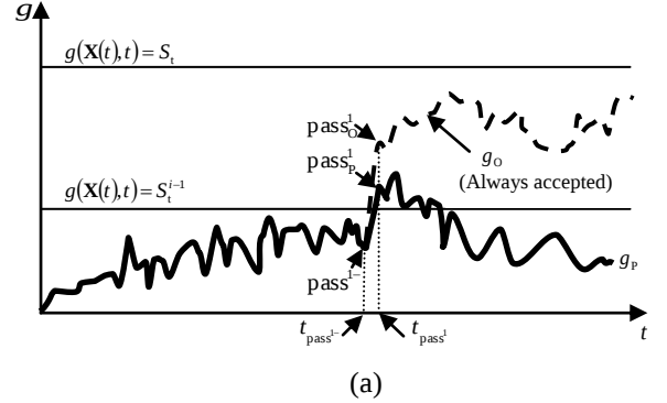
Figure 2. Accepted and rejected sample functions generated by MCMC
