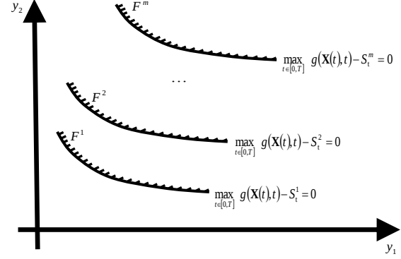
Figure 1. Pictorial representation of failure subdomains
