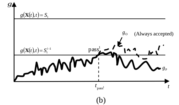
Figure 3. Sample functions generated by splitting
