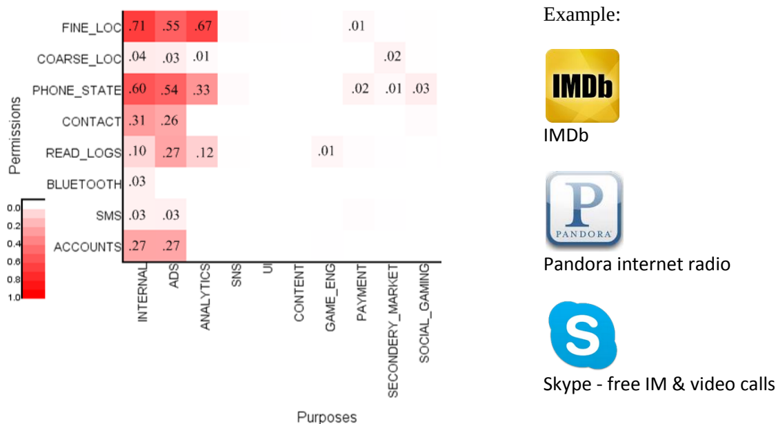
Figure 15: Heat map of cluster 5. This cluster of apps consumes permissions both internally and for delivering targeted ads and facilitating mobile analytics.
