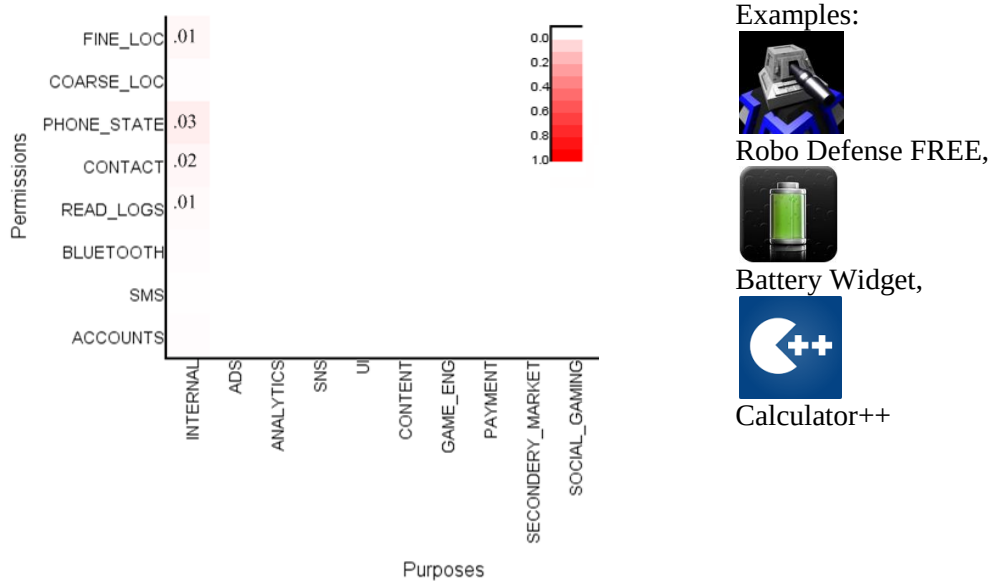
Figure 11: Heat map visualization of the centroid of cluster_1. Permissions are displayed along the vertical axis, while the possible purposes associated with these permissions are displayed along the horizontal axis. Apps in this cluster seldom use any sensitive permissions. More red color indicates a higher proportion of apps requesting a given permission for a particular purpose.
