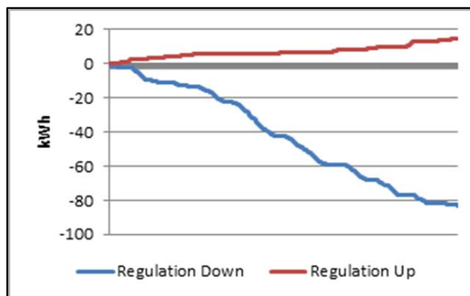
Figure 1. Integrated Automatic Generation Control Signal Illustrating kWh of Energy Throughput Over 24 Hours of Frequency Regulation Response With a 10 kWh Bidirectional Charger
