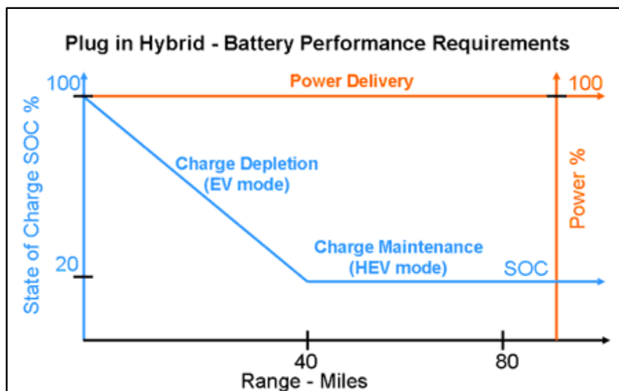
Figure 11. Plug-In Hybrid Electric Vehicle State of Charge Profile (From Woodbank, 2012)
