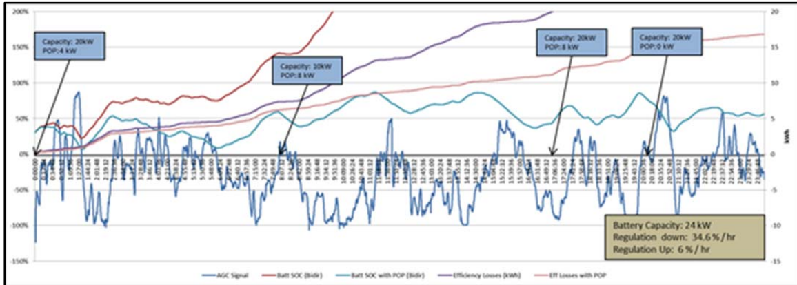
Figure 37. State of Charge Simulation—High Capacity with a Dynamic POP
