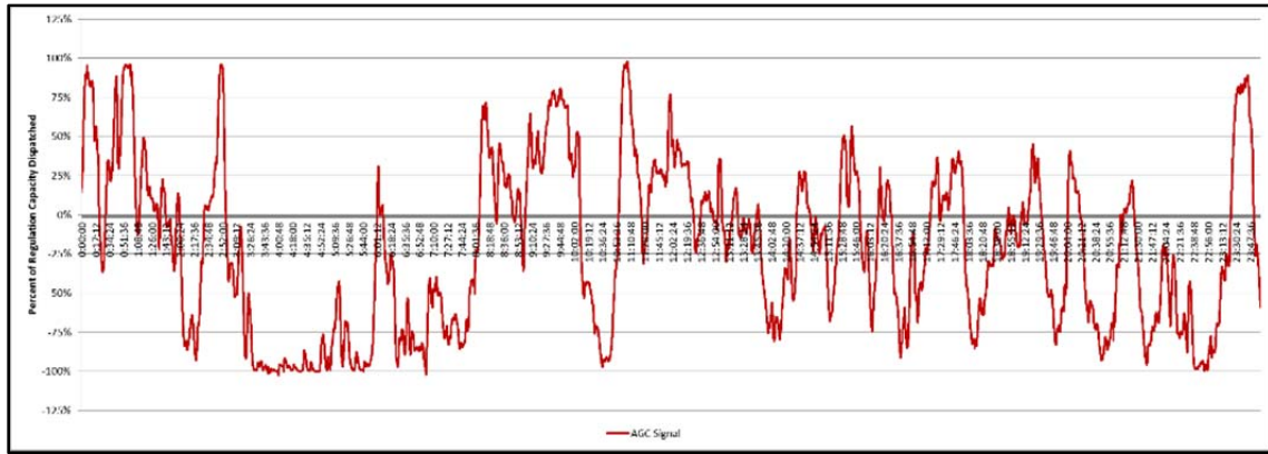
Figure 30. Example Automatic Generation Control Dispatch Signal
