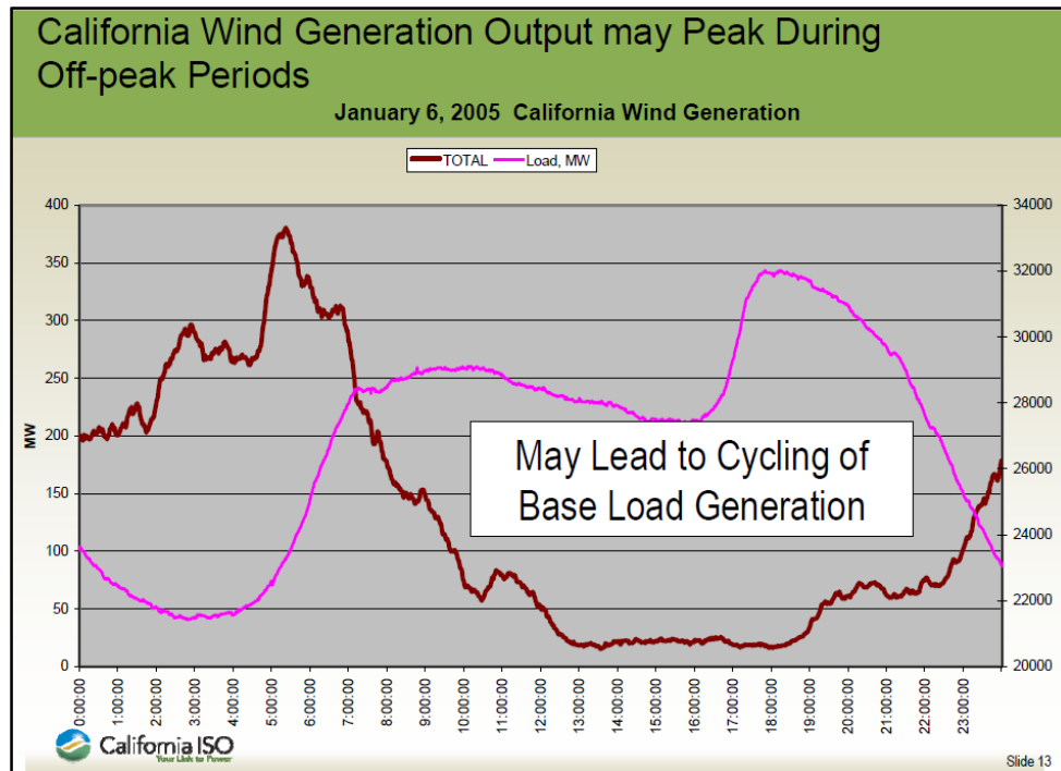
Figure 14. Wind Generation versus Peak Demand (From Helman, 2009)
