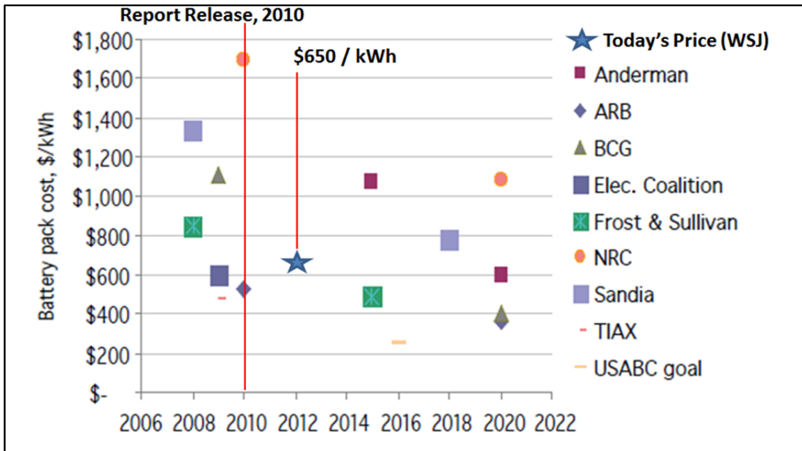
Figure 20. Cost Estimates of Electric Vehicle Battery Packs (From MIT, 2010)
