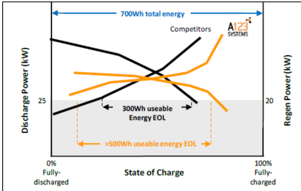
Figure 12. Useable Battery State of Charge (From A123 Systems Inc., 2009)
