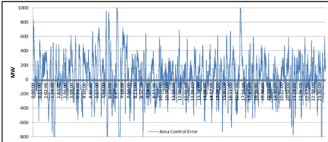
Figure 17. PJM 24-Hour Area Control Error
