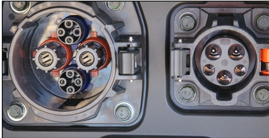
Note. (Left) Level 3 CHAdeMO charge port; (Right) Levels 1 and 2 SAE J1772 charge port
