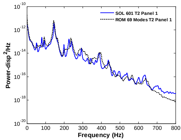
Figure 4.30. Power spectral density of the transverse (T3) and in-plane (T1 and T2) deflections at the middle point of bay 1. Reduced order model and finite element (“SOL 601”), SPL = 136dB .
