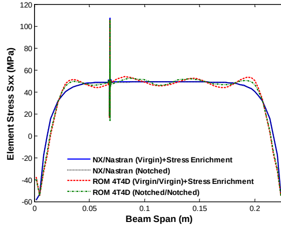
Figure 24. Element stress S_{xx} near the beam edge at y=0, z=h , induced by a uniform pressure of 17kPa. Reduced order model with stress enrichment (“ROM 4T4D+Stress Enrichment”), nonlinear static FEA (“NX/Nastran”).
