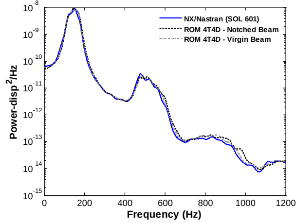
Figure 27. Power spectral density of the transverse displacement at the beam middle point, x=1/2L , y=0 , z=h ( OASPL = 147\text{dB} ). Reduced order model (“ROM(4T4D)”) and FEA (“NX/Nastran”).
