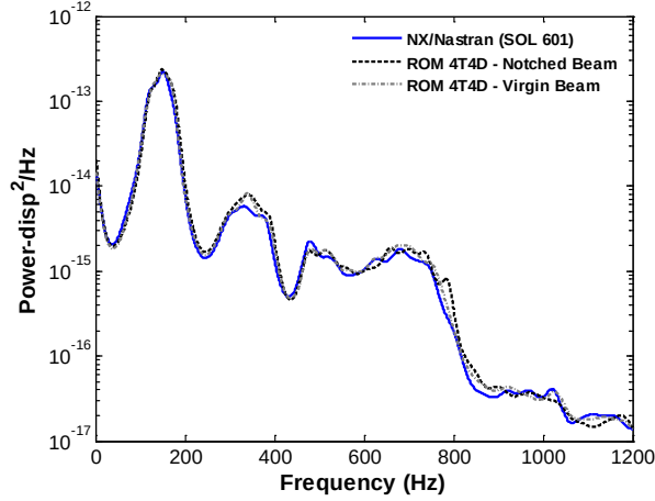
Figure 29. Power spectral density of the in-plane displacement at the beam quarter point, x=1/4L , y=0 , z=h ( OASPL = 147\text{dB} ). Reduced order model (“ROM(4T4D)”) and FEA (“NX/Nastran”).
