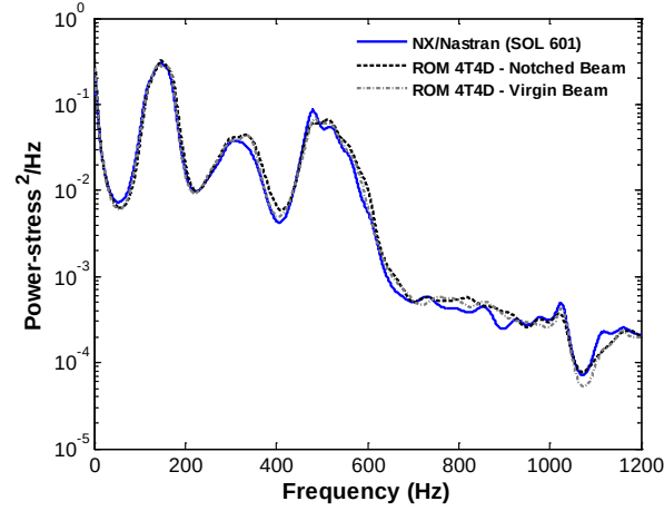
Figure 30. Power spectral density of the S_{xx} element stress near the middle of the beam at y=0 , z=h (OASPL = 147dB). Reduced order model (“ROM(4T4D)”) and FEA (“NX/Nastran”).
