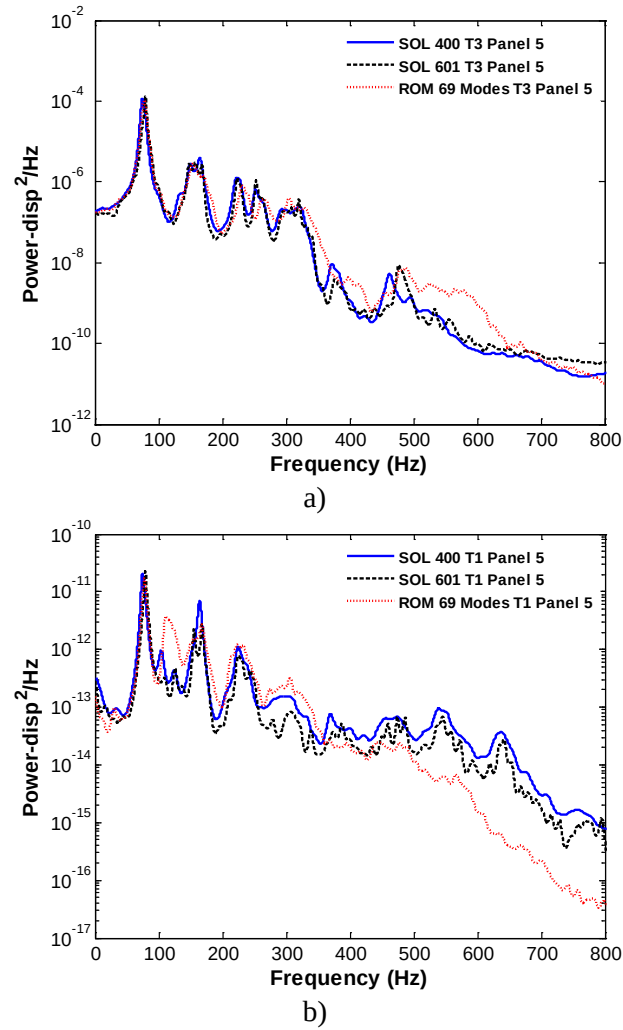
Figure 4.38. Power spectral density of the transverse (T3) and in-plane (T1) deflections at the middle point of bay 5. Reduced order model and finite element (“SOL 400” and “SOL 601”), SPL =144dB.
