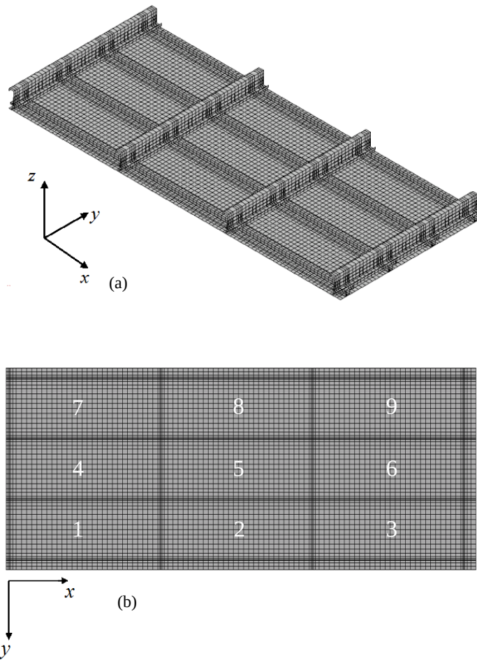
Figure 4.2. Finite element model of the 9-bay fuselage sidewall panel, (a) isometric view, (b) top view.
