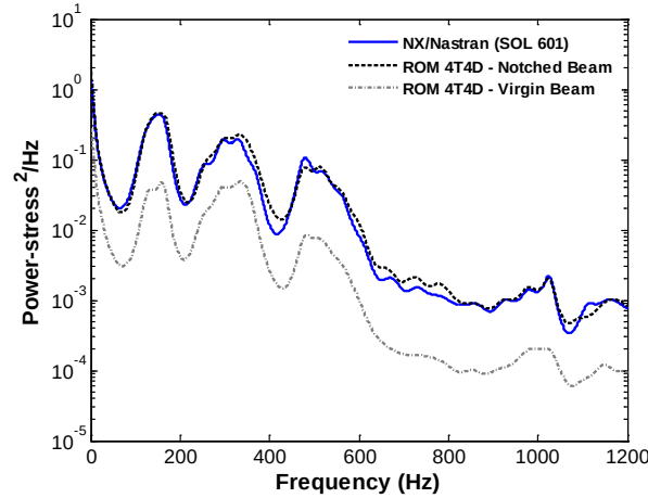
Figure 32. Power spectral density of the S_{xx} element stress near the notch at y=0 , z=h (OASPL = 147dB). Reduced order model (“ROM(4T4D)”) and FEA (“NX/Nastran”).
