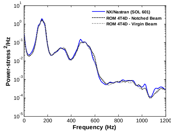
Figure 31. Power spectral density of the S_{xx} element stress near the support of the beam at y=0 , z=h (OASPL = 147dB). Reduced order model (“ROM(4T4D)”) and FEA (“NX/Nastran”).
