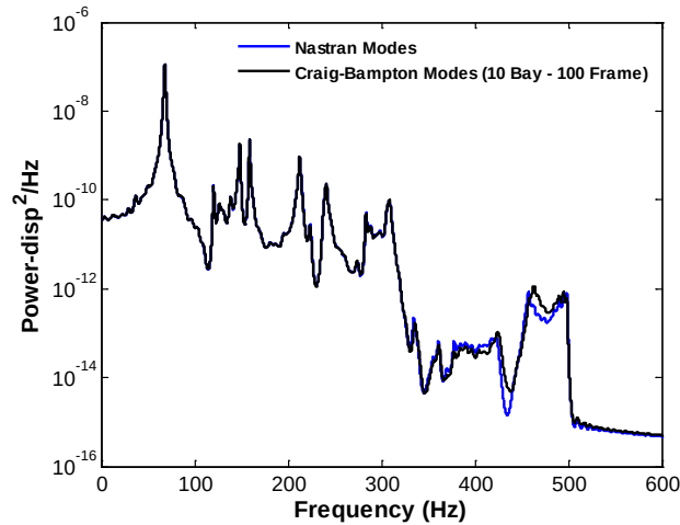
Figure 4.54. Power spectral density of the transverse (T3) deflection at the middle point of bay 5. Craig-Bampton model and finite element (“Nastran Modes”), SPL = 106dB .
