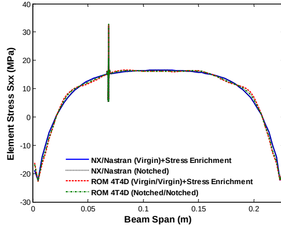
Figure 23. Element stress S_{xx} near the beam edge at y=0, z=h , induced by a uniform pressure of 2.6kPa. Reduced order model with stress enrichment (“ROM 4T4D+Stress Enrichment”), nonlinear static FEA (“NX/Nastran”).
