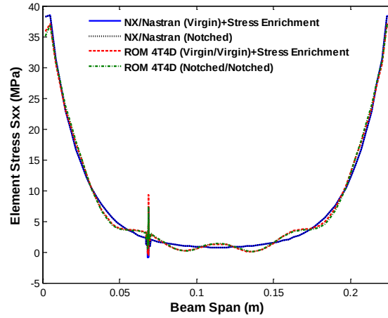
Figure 25. Element stress S_{xx} near the beam edge at y=0, z=h , induced by a uniform pressure of - 2.6kPa. Reduced order model with stress enrichment (“ROM 4T4D+Stress Enrichment”), nonlinear static FEA (“NX/Nastran”).
