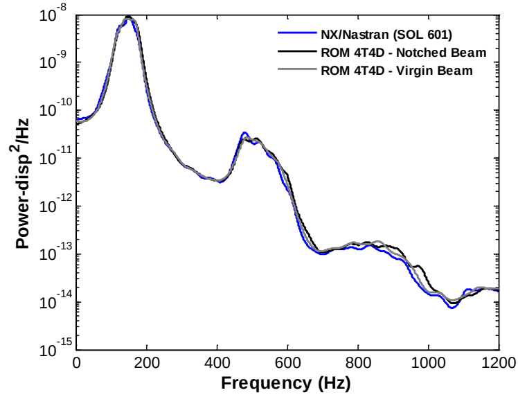
Figure 5.27. Power spectral density of the transverse displacement at the beam middle point, x=1/2L , y=0 , z=h ( OASPL = 147\text{dB} ). Reduced order model (“ROM(4T4D)”) and FEA (“NX/Nastran”).
