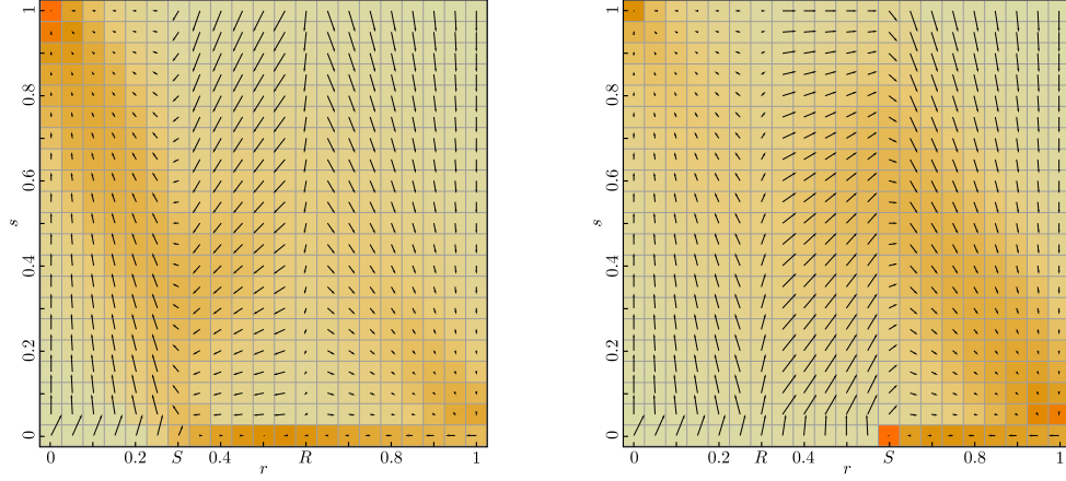
Figure 3: Mean flow fields in (r, s) space for the two cases R > S (left) and S > R (right), using N = 20 . Colors represent the total amount of time spent at a cell, ranging from light gray (little time) to bright orange (much time), assuming a uniform initial distribution on the number of players of each strategy type. For R > S , all trajectories eventually end in Dystopia. For S > R , we have treated r = S as an absorbing point (all trajectories passing through that point actually cycle near it indefinitely), so that all trajectories end either there or at Dystopia.
