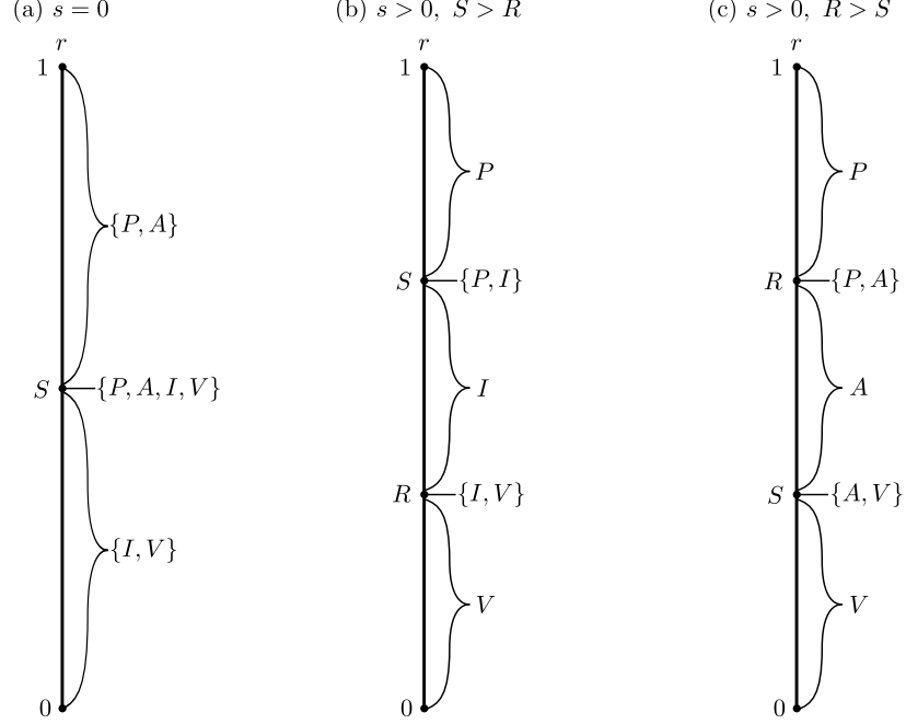
Figure 1: A graphical representation of the best response function BR_i(s, r) under the three cases: (a) s = 0 , (b) s > 0 , S > R , and (c) s > 0 , R > S .
