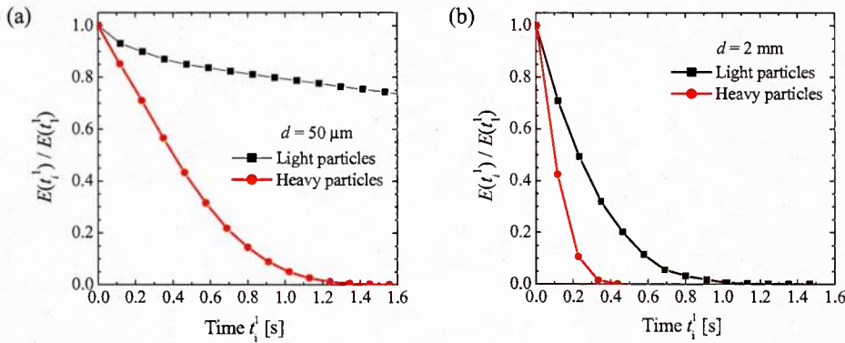
Figure 7. Comparison of energy decay between light and heavy particles of diameter 50 \mu\text{m} (a) and 2 \text{ mm} (b).
