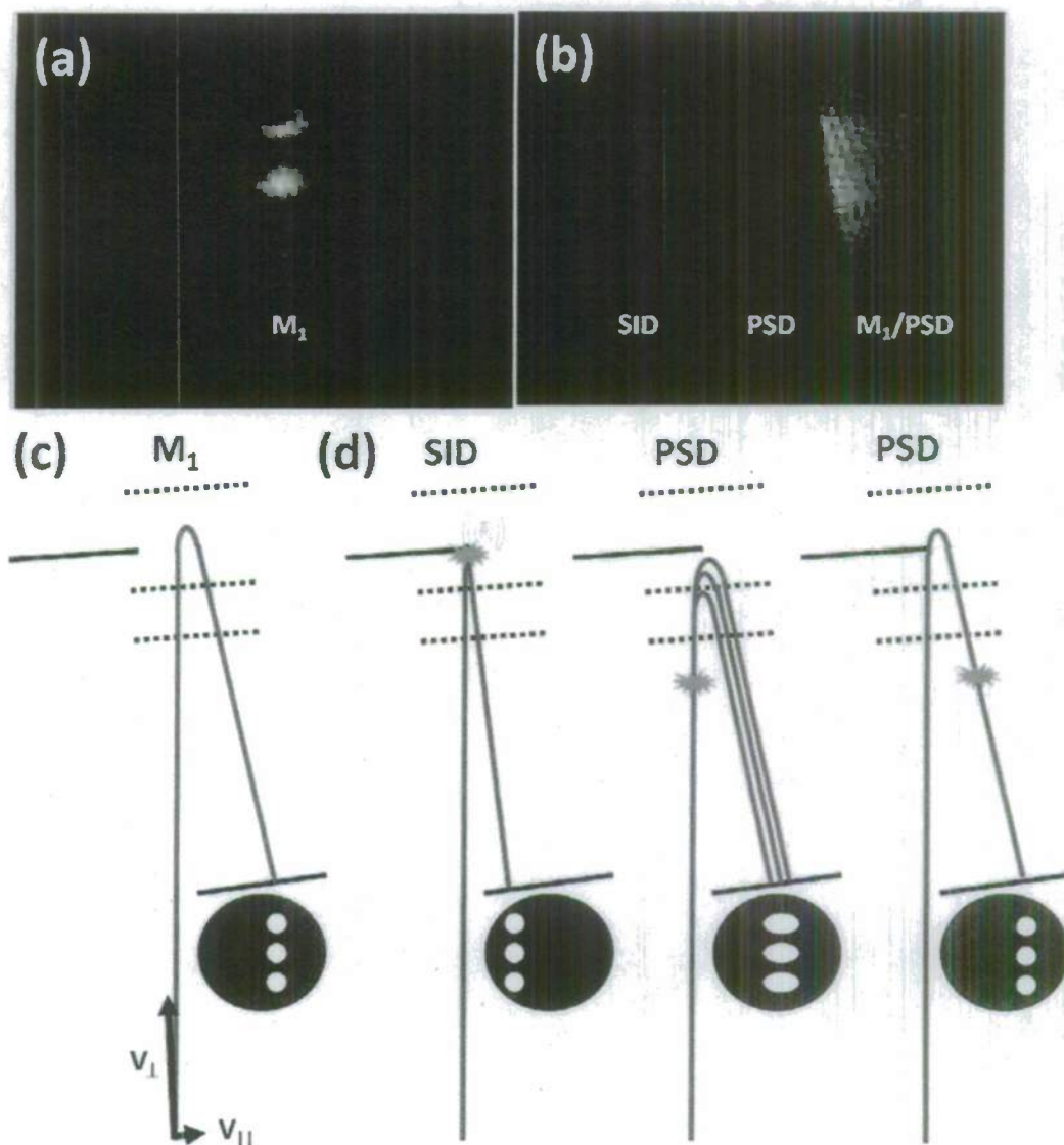
Figure 5: Schematic of the experiment. Two-dimensional images of triply charged angiotensin I (433 amu) with the SID surface (a) withdrawn and (b) inside the reflectron. Illustrations showing the trajectories and arrival patterns at the detector of (c) precursor ions and (d) three fragmentation processes: SID, PSD pre-reflectron, and PSD post-reflectron. PSD does occur inside the reflectron but is spread in position and time between pre- and post-reflectron PSD signals.
