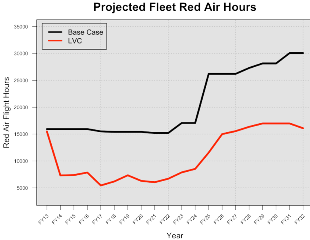
Figure 28. Fleet hours expended performing the red air mission as prescribed by ADSOT for LVC range excursion compared to base case.
