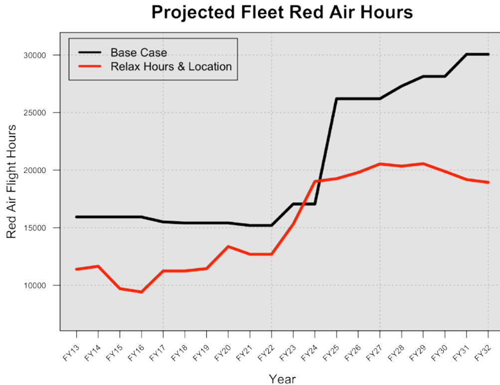
Figure 25. Fleet hours expended performing the red air mission as prescribed by ADSOT in the relaxed constraint excursion. Total savings of 105,000 hours are realized over the entire planning horizon.
