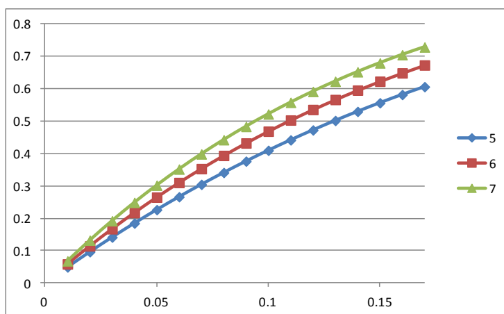
Figure 4. Graph of probability of success per day versus coverage Pdt and number of launches
