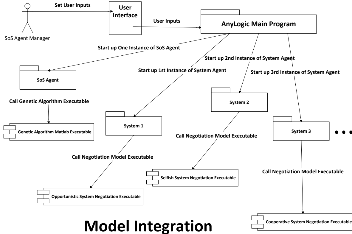
Figure 32. Overall Agent-Based Implemented Model Architecture
