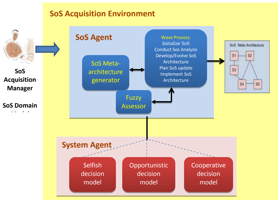
Figure 3. Overall Agent-based Model Architecture
