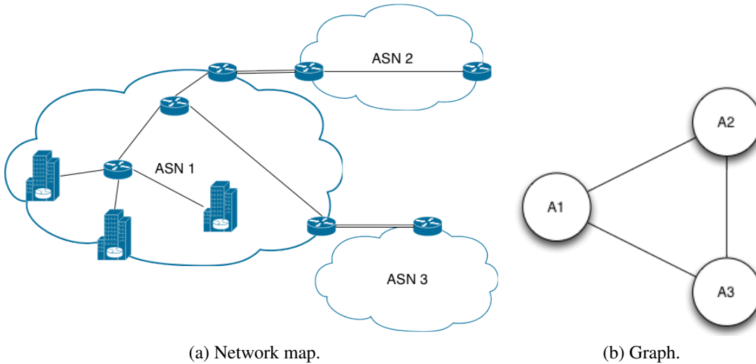
Figure 2.2: AS-level representations.
