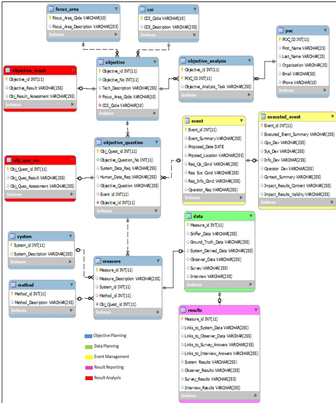
Figure 5. iFIRE Entity Relationship Diagram.
