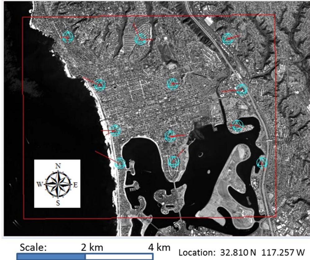
Figure 22. WV1 background image showing ground space residual analysis results of the triangulation adjustment that controlled the WV-1 stereo triplet to the LiDAR data. The RMS was 0.6 meters
