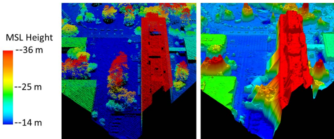
Figure 31. Split screen close up view of the LiDAR data on the left and the stereo image collected point cloud on the right showing many unique differences. The LiDAR data is very clean and sharp (Left) and the Stereo point cloud is interpolated and rough in areas (Right).
