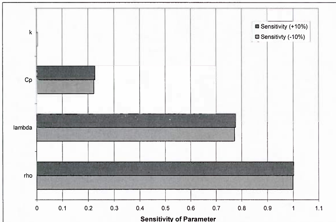
Figure 7. Positive and negative sensitivities of failure time to relevant physical parameters.
