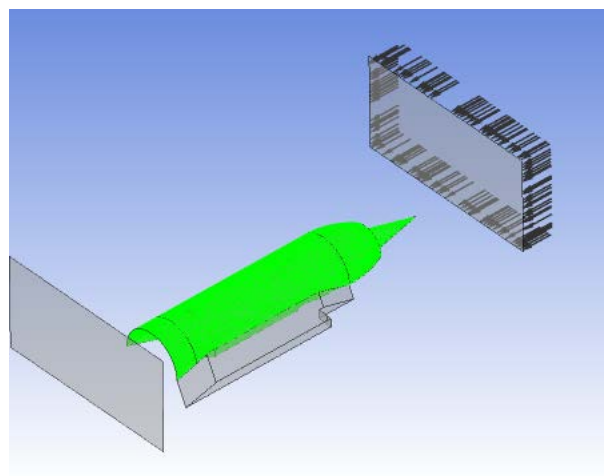
Figure 42 Ramjet boundary.
