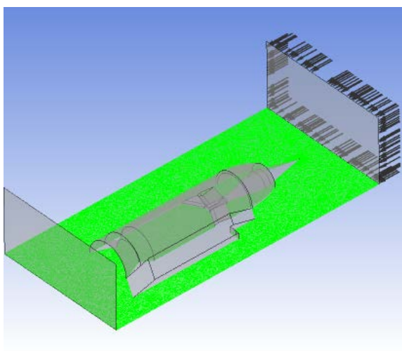
Figure 40 Symmetry boundary.
