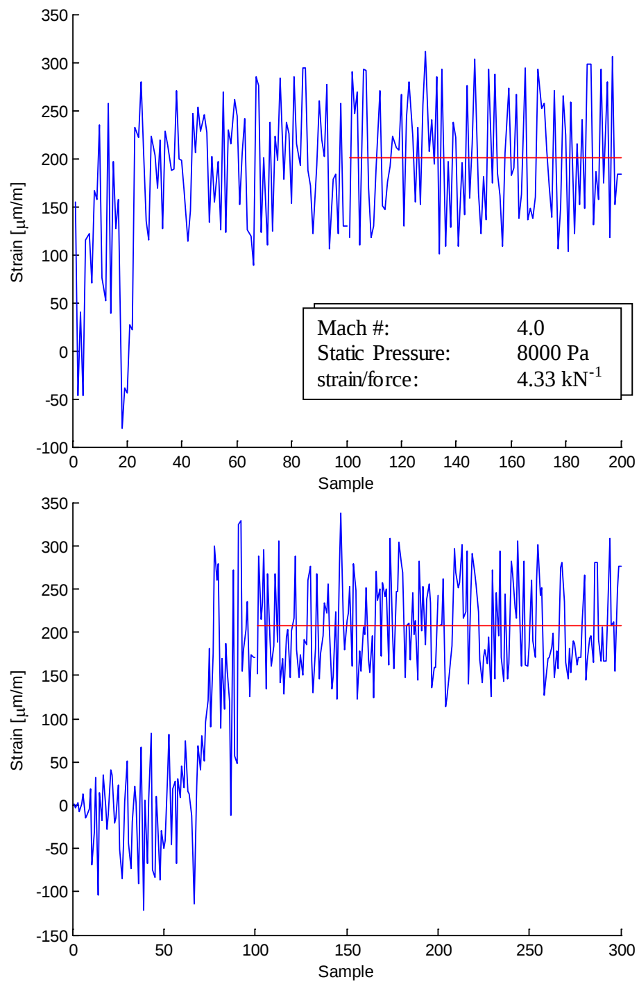
Figure 11 Strain readings from SSWT run with Nozzle C.
