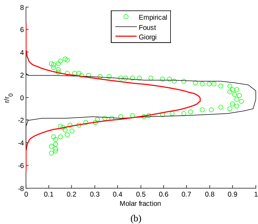
Figure 22 Molecular Oxygen mole fraction profiles at (a) 25.4 mm and (b) 124 mm from the inlets. After [4].
