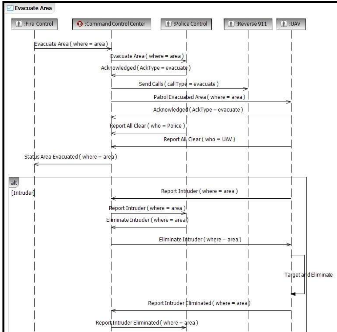
Figure 10: RACRS Evacuate Area Sequence Diagram
