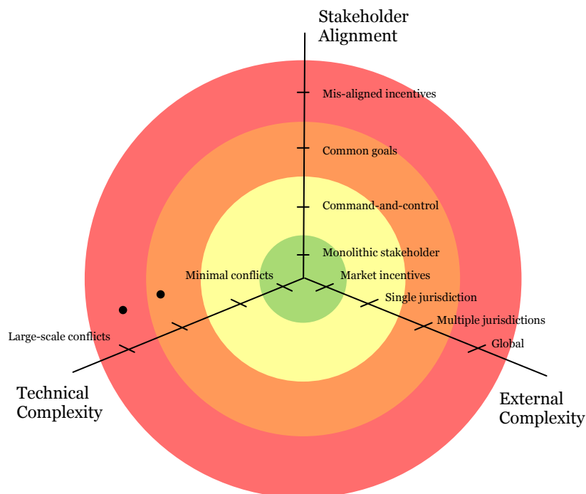
Figure 3: Integration Taxonomy
