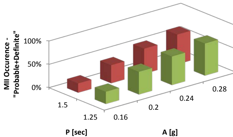
Figure 6. Sway + Roll motion. 3-D figures of MII occurrence (“Probable,” “Definite,” and “Probable + Definite”) by peak sway acceleration and period
