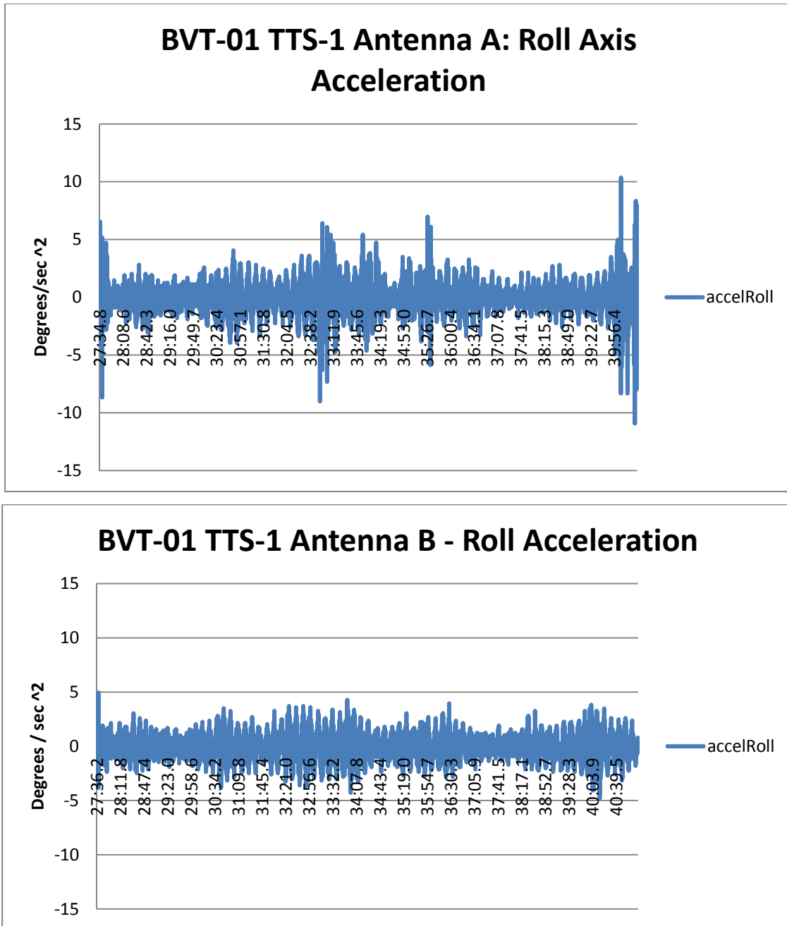
Figure 16. Comparison plots of roll axis acceleration during the BVT-01 event (From TTS-1, Jun 2010)
