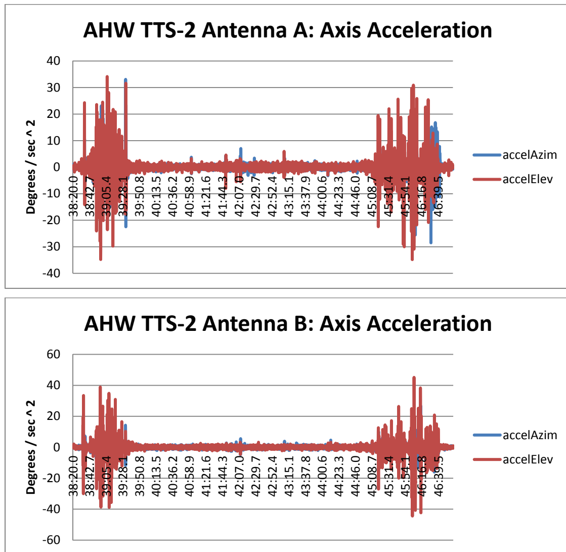
Figure 23. Azimuth and Elevation axis acceleration comparisons for the AHW mission event (From TTS-2, 2011)
