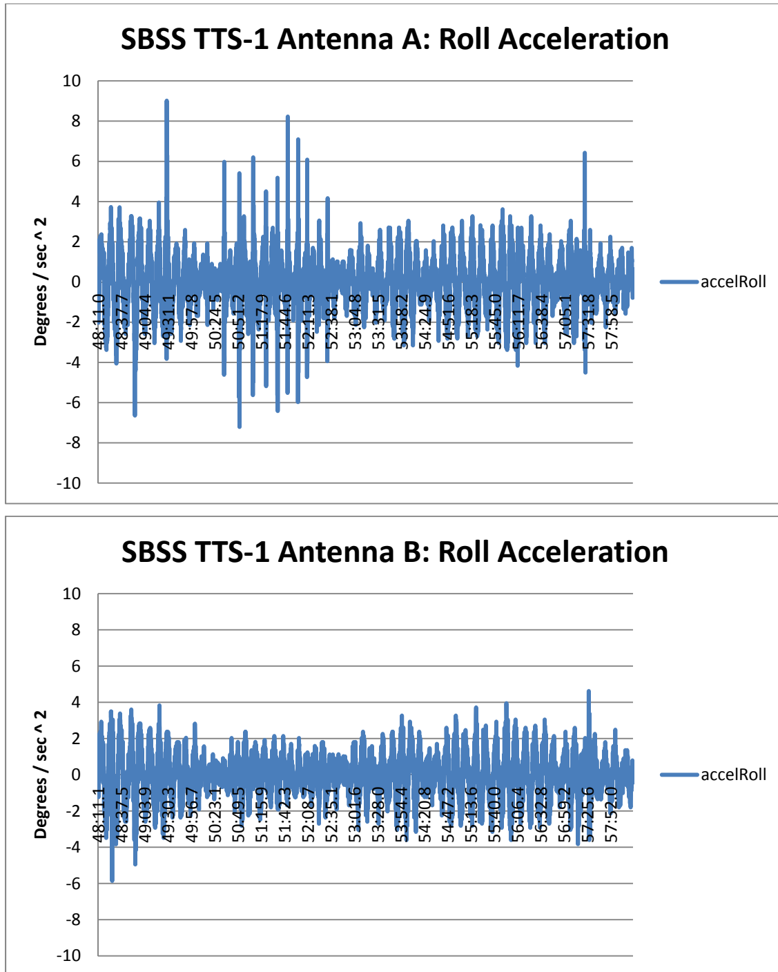
Figure 20. Roll axis acceleration plots for the SBSS mission event (From TTS-1, Oct 2010)
