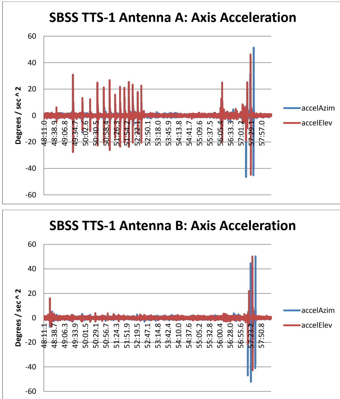
Figure 19. Axis acceleration plots for the SBSS mission event (From TTS-1, Oct 2010)
