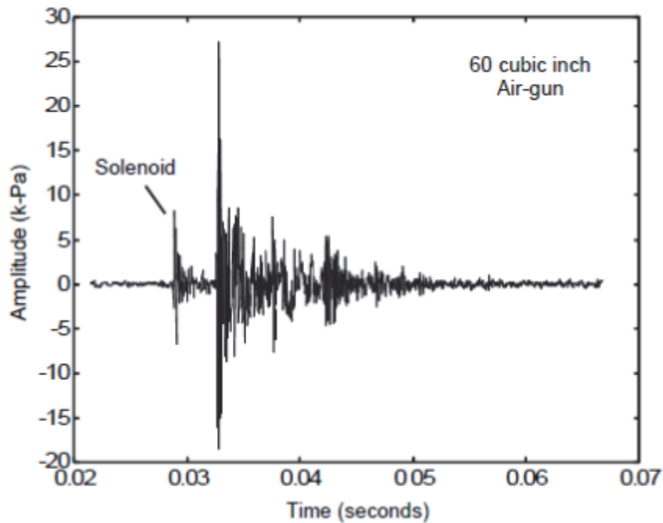
Figure 8. Characteristic Waveform of an Airgun Pulse
