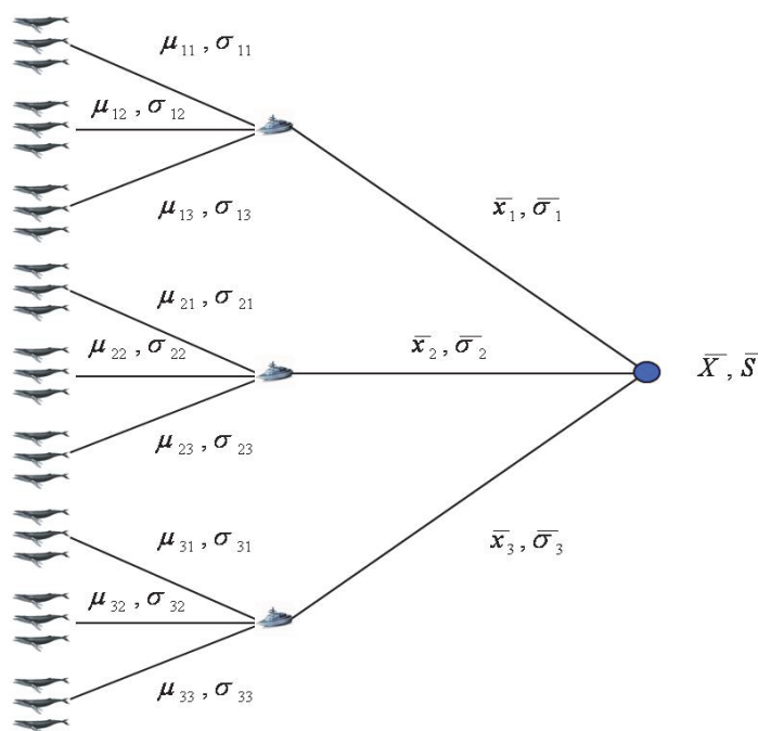
Figure 27. Bootstrapping Approach Used to Calculate Simulation Statistics
