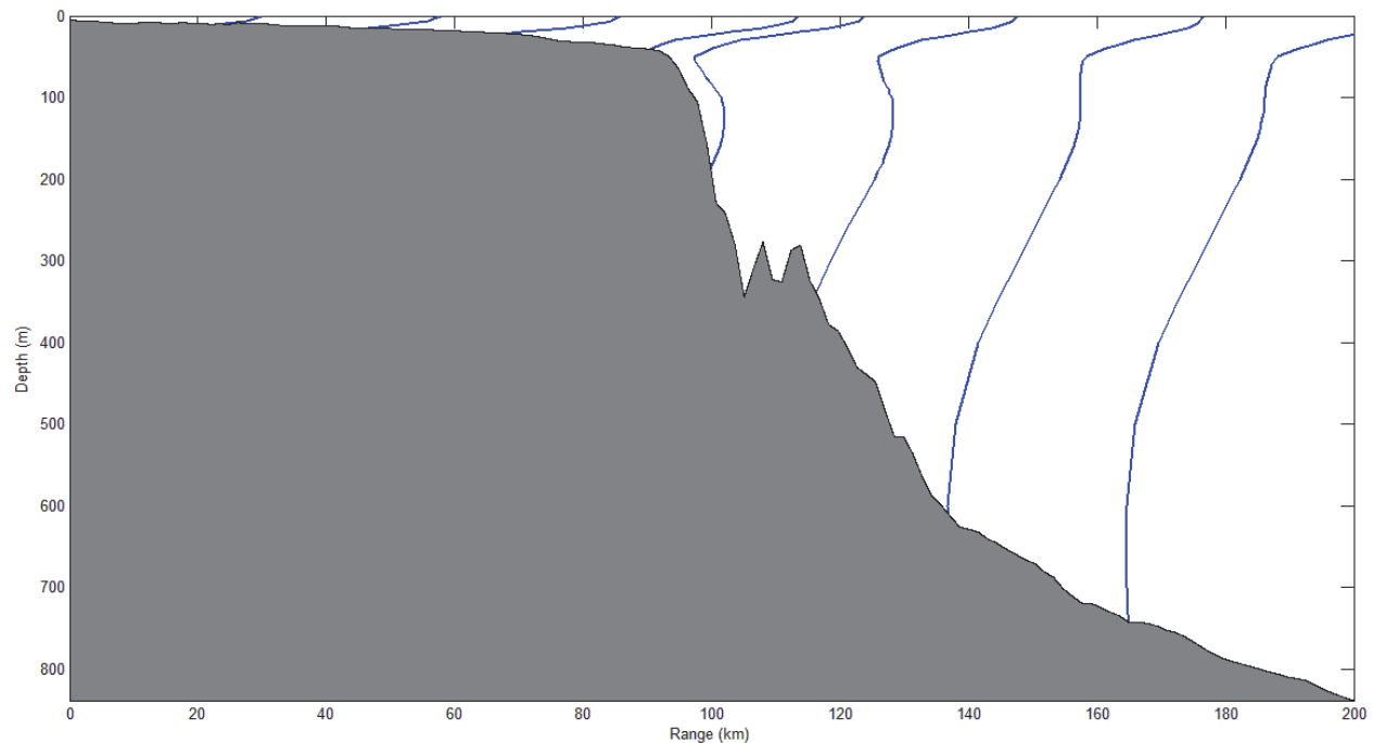
Figure 18. Sample Sound Speed Profiles
