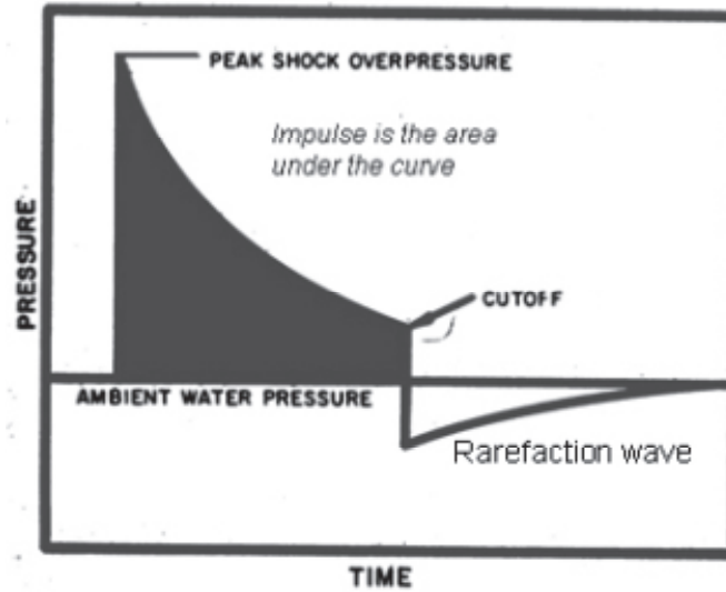
Figure 19. Generalized Shock Wave
