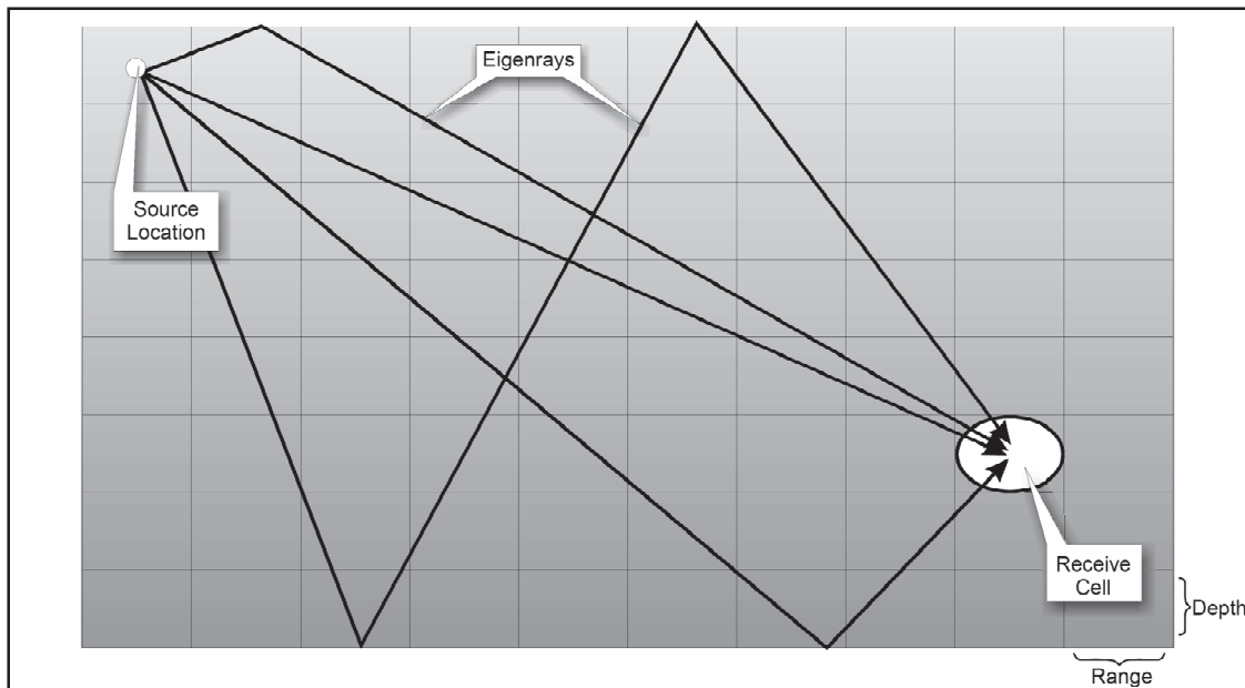
Figure 21. Typical Eigenray Paths for Relatively Short-Range Propagation
