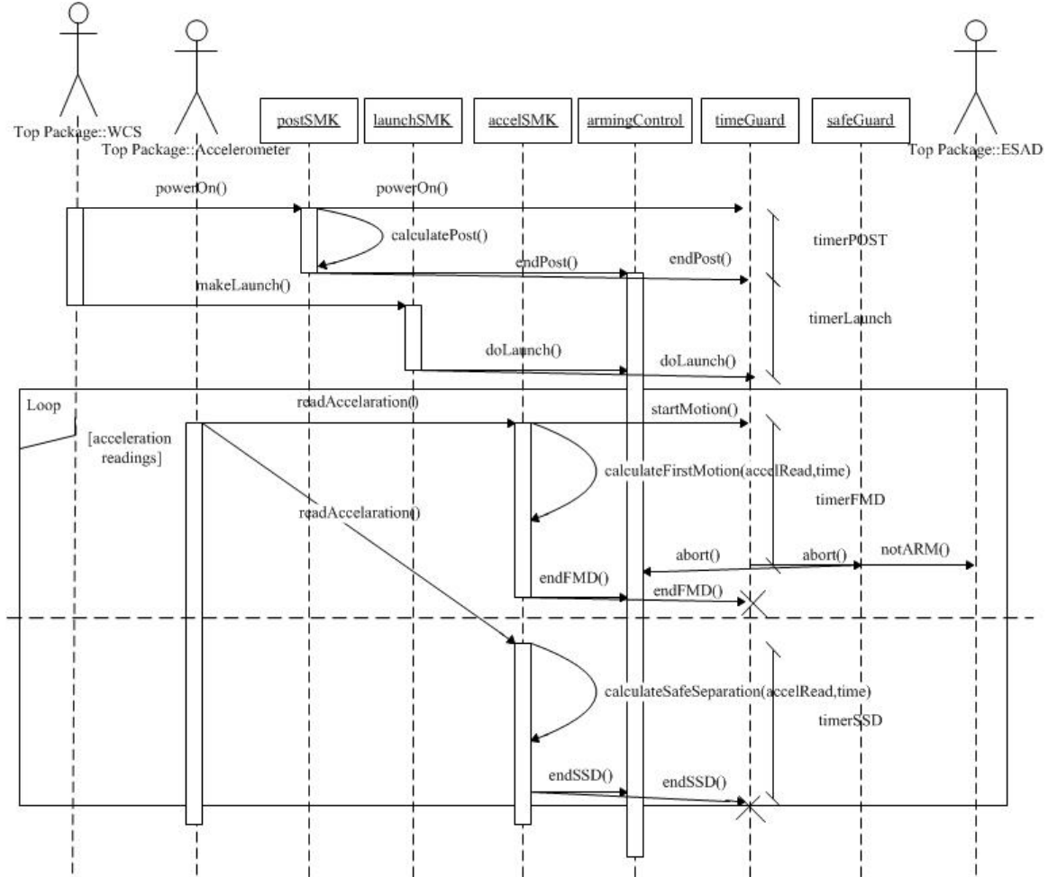
Figure 17. Sequence diagram for ESAD to remain in safe state.
