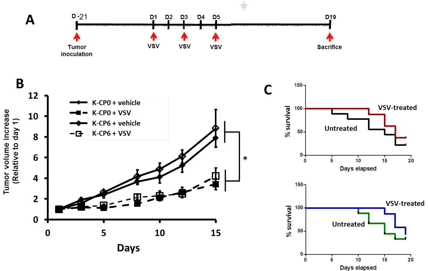
Figure 3: Antitumor activity of VSV against cisplatin resistant tumors in vivo . A) Flowchart describing the schedule and time points for the animal procedures. B) Oncolytic activity of VSV against K-CP0 or K-CP6 cells in DBA/2 mice (n=8) injected with respective tumor cells and treated as described in A). C) Estimation of survival based on the Kaplan-Meier analysis. Top diagram represents survival of mice injected with K-CP0 cells and bottom diagram represents mice injected with K-CP6 cells. Respective treatments are indicated next to the curves. * p < 0.05
