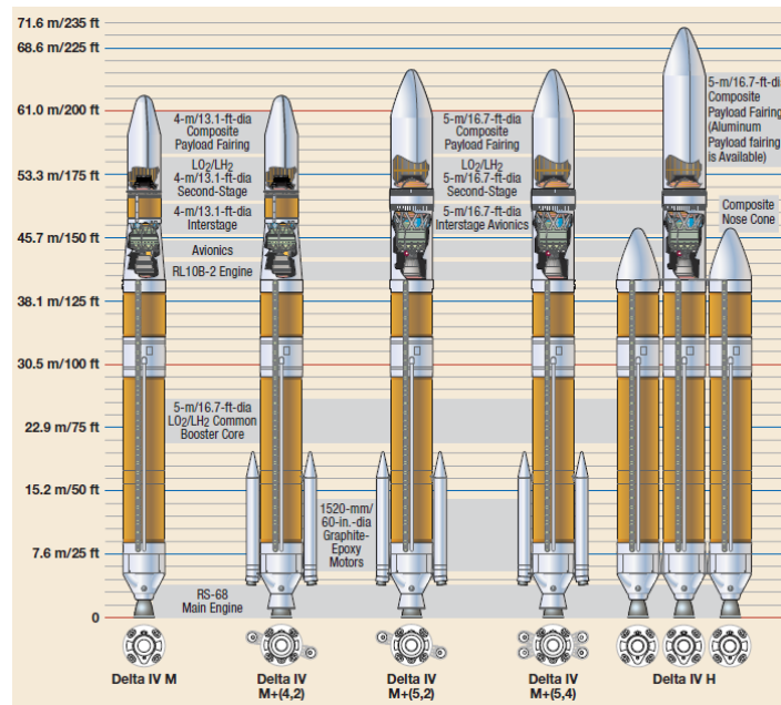
Figure 12. Delta IV Configurations (from United Launch Alliance, 2007)
