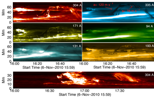
Fig. 4. Time-distance diagrams along cut 1 (see panel i of Fig. 3) show the simultaneous upward motions of the eruption and downward streams in different AIA bandpasses. The red dotted line in the top right panel is the parabolic fit to the moving features. The corresponding accelerations are also shown. The bottom panel is a time-distance diagram taken along cut 4 (see panel i ) of Fig. 3), showing the downward motions of the apex plasma.
