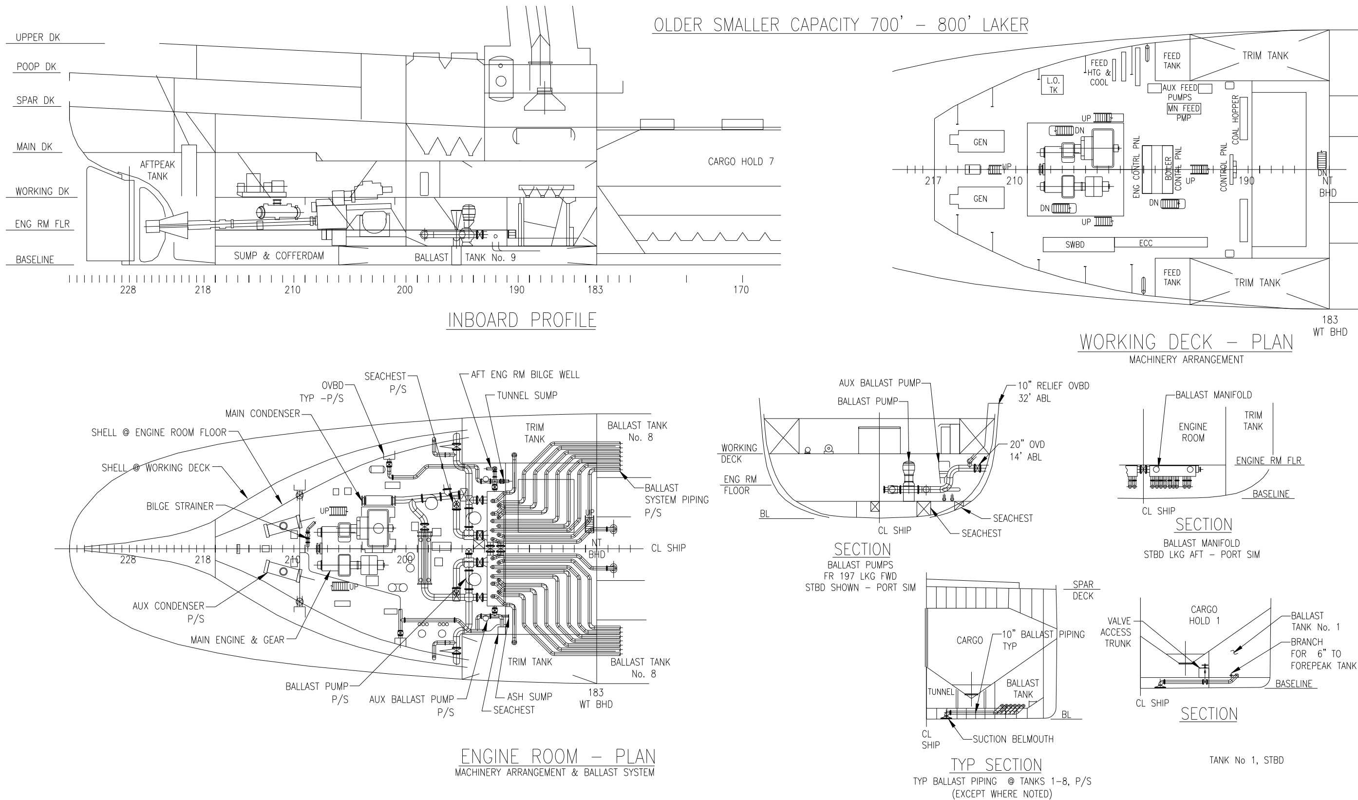
Figure C-3. Older, small capacity 700' - 800' Laker: engine room arrangement.
