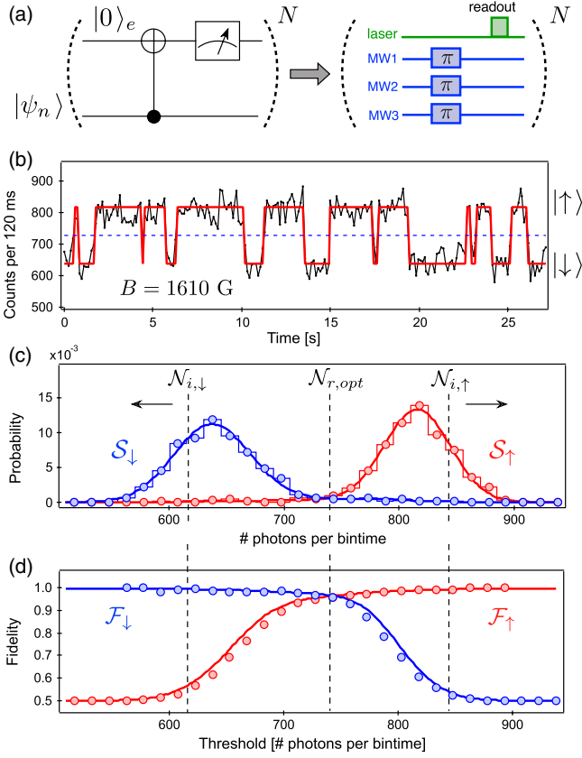
Figure from Phys. Rev. Lett. 110, 060502 (2013).
