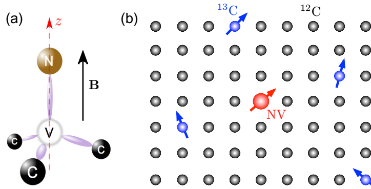
Figure A1. (a) Atomic structure of the NV defect in diamond. (b) Schematic view of a single NV defect (red arrow) placed in a nuclear-spin bath. Blue arrows indicate ^{13}\text{C} nuclear spins located randomly in the diamond lattice. Decoherence of the central electronic spin is induced by hyperfine coupling with the ^{13}\text{C} nuclear spins.
