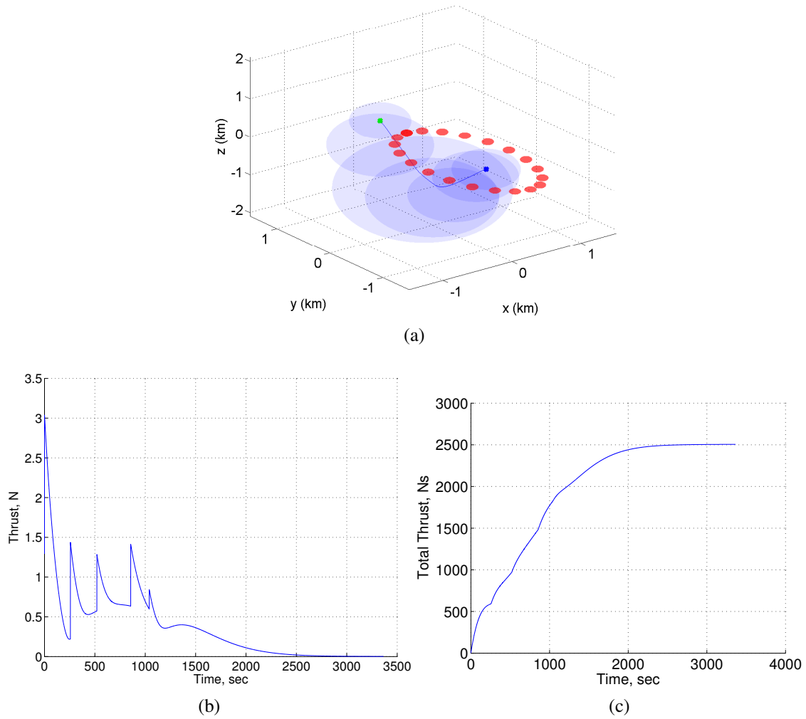
Figure 7: (a) Debris avoidance path for a non-stationary debris using the union method. (b) The time history of thrust magnitude. (c) Cumulative thrust vs time.
