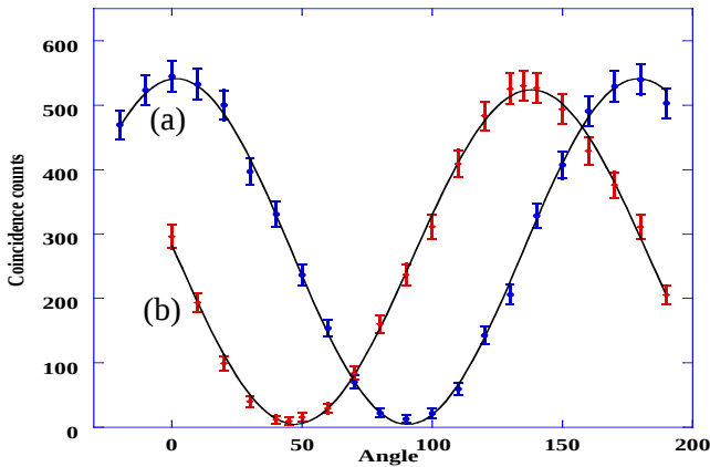
Fig. 3. Two-photon interference fringes with HNLF at 77° K (a) \theta_1 = 0^\circ and (b) \theta_1 = 135^\circ .
