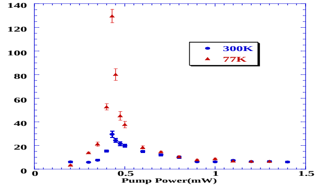
Fig. 2. Coincidence count to accidental coincidence count ratio (CAR) versus pump power with HNLF at 300° K (Blue dot) and 77° K (Red triangle).
