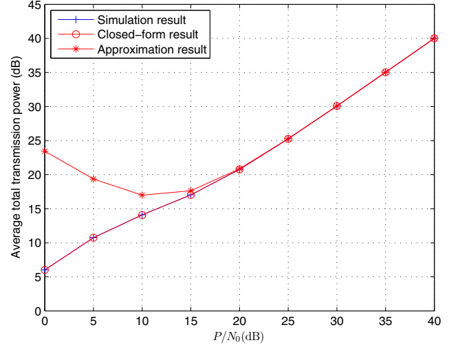
Fig. 2. Average total power consumption per information packet, P_{s,l} = P_r = P , 1 \leq l \leq 4 , \gamma_0 = 10 dB, L = 4 .
