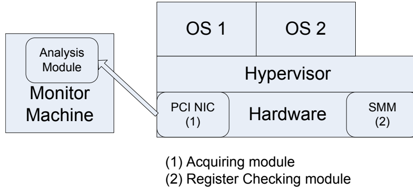
Fig. 2: The architecture of HyperCheck
