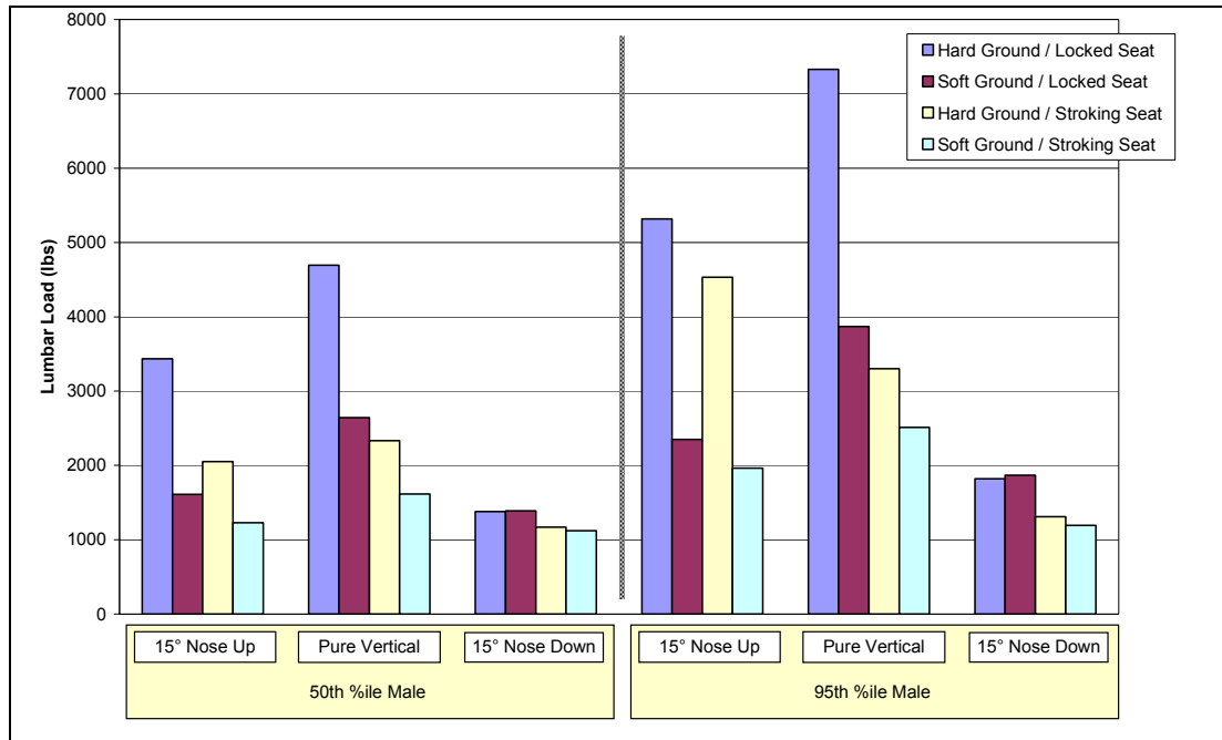
Figure 15. Lumbar force resultant experienced by medium and large manikins under different impact conditions.
