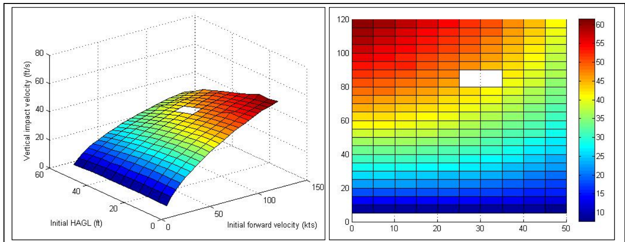
Figure 3. Surface plot with the poorly converged data point removed. Note: This improves the contrast evident in the colormap (right) when the range of impact velocities is narrowed.
