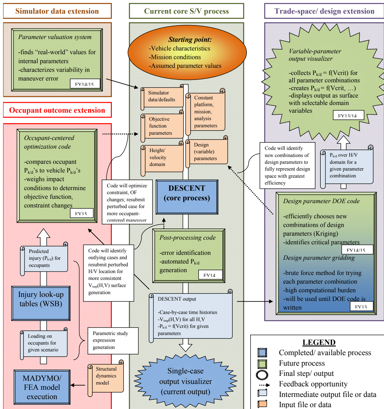
Figure 21. DESCENT data flow diagram including proposed extensions.
