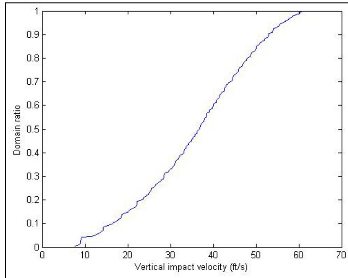
Figure 6. Domain ratio plot.
