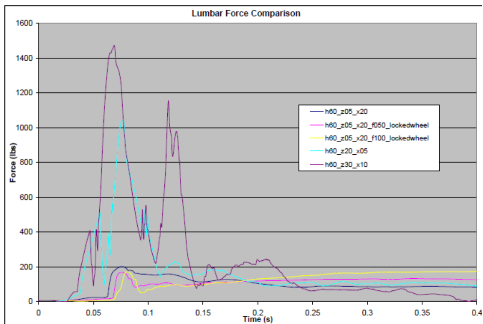
Figure 14. Lumbar force resultant experienced by the manikin under different impact conditions.
