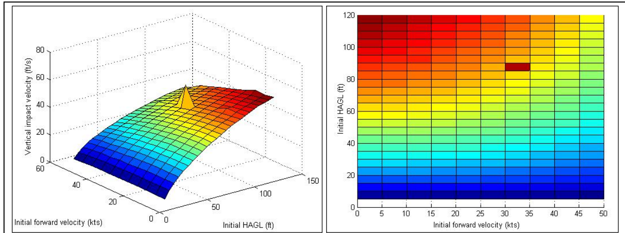
Figure 2. Surface plot of vertical impact velocity over the analysis domain for a total-power-loss scenario. Note: Although any combination of state variables can determine kill category, vertical impact velocity is the typical quantity, displayed here. Each grid vertex (data point) represents a separate optimization done by the code. Note that one H/V location displays particularly poor convergence.
