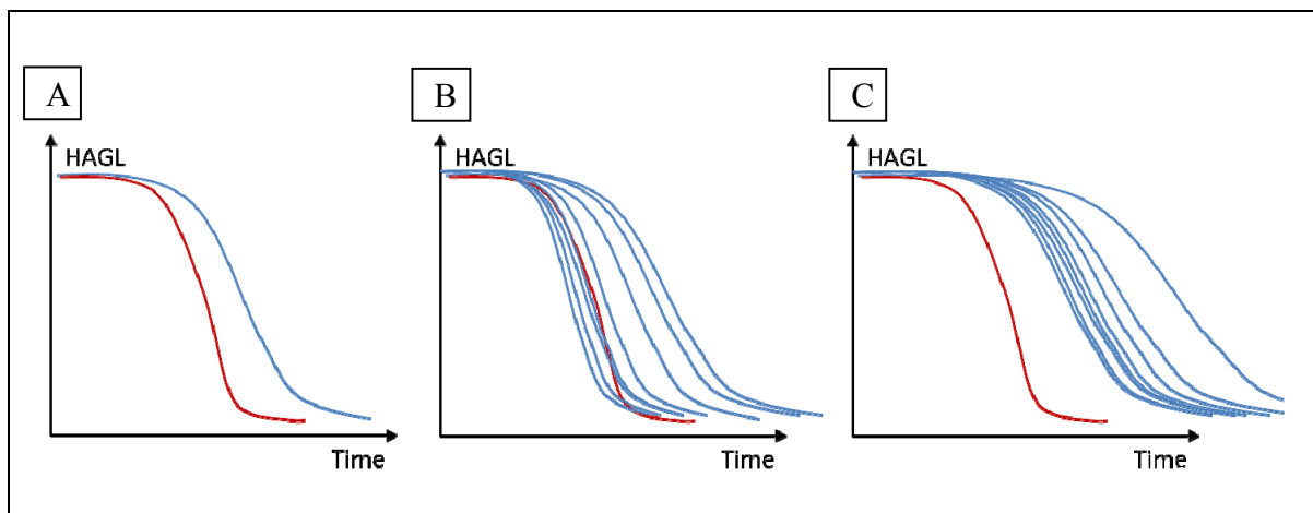
Figure 7. Hypothetical plots of HAGL vs. time for DESCENT output (red) and validation data (blue). Note: With only limited flight test data (plot A, left), it is difficult to tell whether somewhat differing results are actually divergent. Using simulator data, it becomes apparent whether the DESCENT solution is within the range of plausible solutions (plot B, center), or outside of it (plot C, right).
