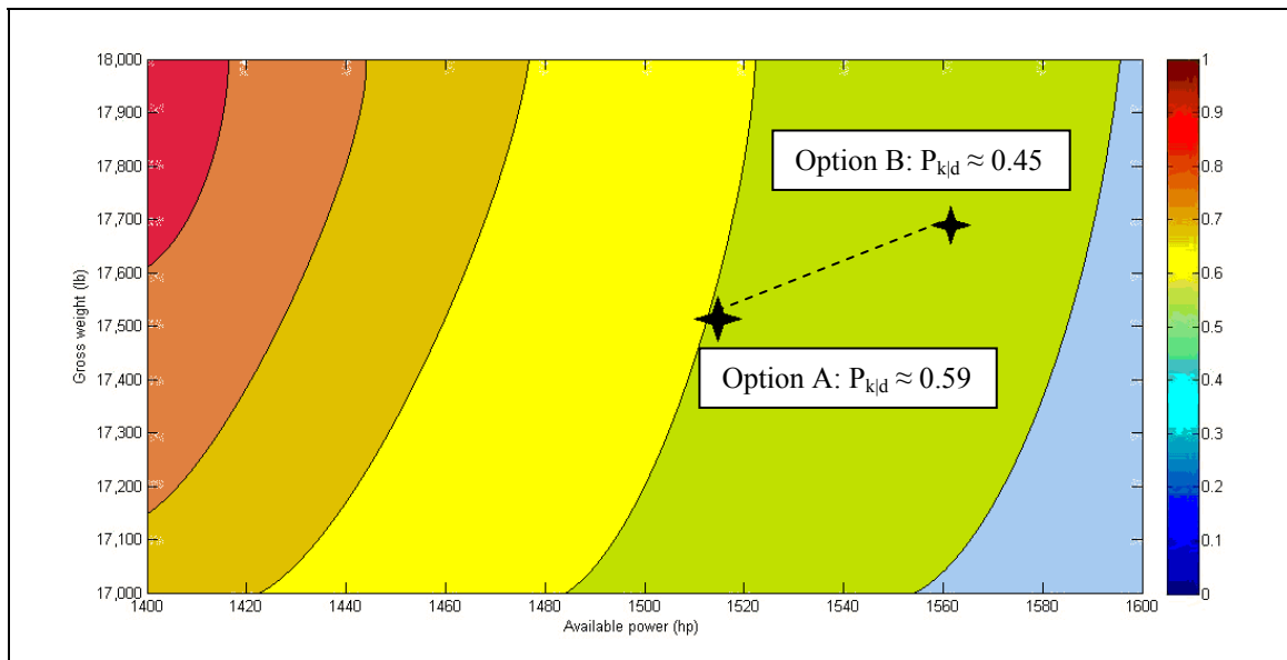
Figure 19. Engine options A and B on the P_{k|d} vs. power and weight surface plot.
