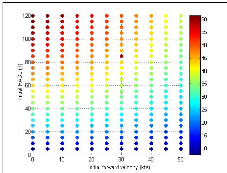
Figure 4. 3-D scatterplot of the same output. Note: This example is rotated to mimic a typical H/V diagram. The colormap legend, as before, represents vertical impact velocity in ft/s.
