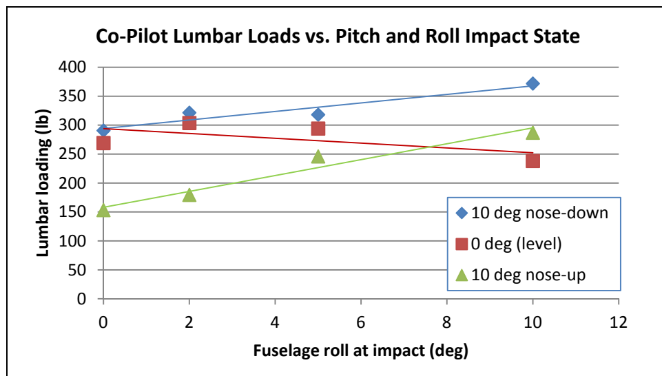
Figure 11. Lumbar loading due to impact.
