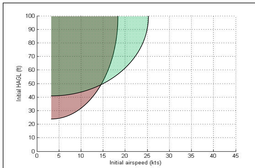
Figure 12. Kill region comparison.
