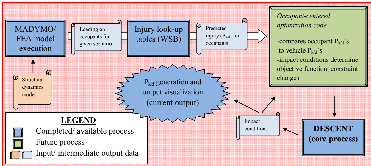
Figure 13. Occupant outcome data flow diagram.
