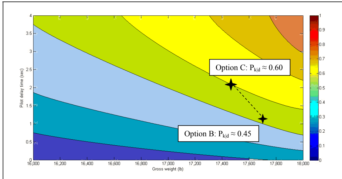
Figure 20. Engine options B and C on the P_{k|d} vs. delay and weight surface plot.
