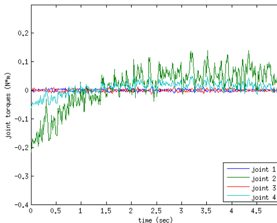
Figure 6: Joint torques commanded by the ID controller in the presence of measurement noise ( \sigma = 0.15^\circ ).
