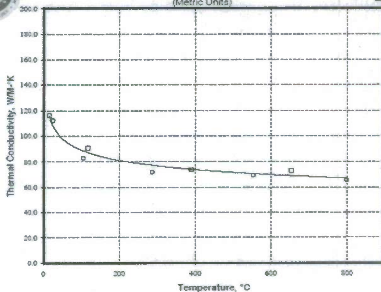
Thermal Conductivity of LaB 6 -ZrB 2 Rod Specimens (Metric Units)
