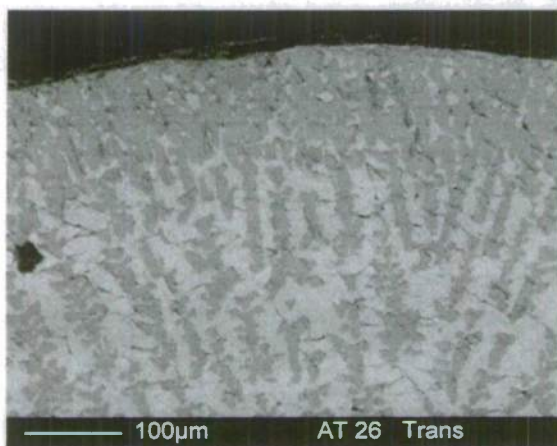
Figure 5: SEM images of sample AT26 (26 mol % \text{TiO}_2 ) a) longitudinal and b) transverse sections showing closely packed dendrites in the outer rim an variation of the orientation of the dendrites. c) A whiter interphase is observed (arrows) between dendrites and matrix.
