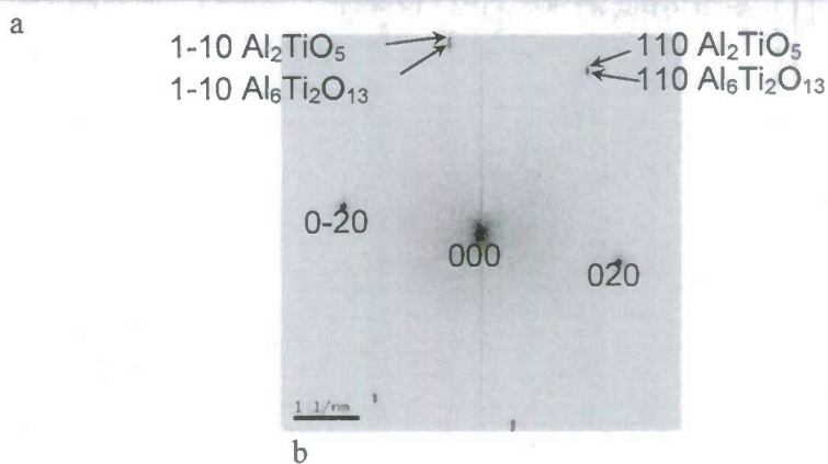
Figure 10: (a) High resolution image of AT44 in [001] zone axis across a \text{Al}_2\text{TiO}_5 and \text{Al}_6\text{Ti}_2\text{O}_{13} interface b) associated FFT: the 110 reflections for \text{Al}_2\text{TiO}_5 and \text{Al}_6\text{Ti}_2\text{O}_{13} do not overlap.
