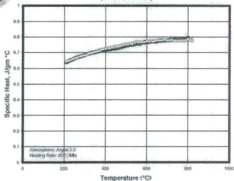
Specific Heat of Lab6-ZrB 2 Rod Specimens (Metric Units)
