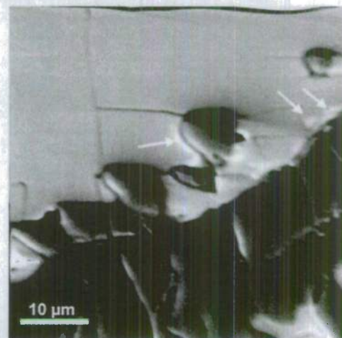
Figure 5: SEM images of sample AT26 (26 mol % \text{TiO}_2 ) a) longitudinal and b) transverse sections showing closely packed dendrites in the outer rim an variation of the orientation of the dendrites. c) A whiter interphase is observed (arrows) between dendrites and matrix.
