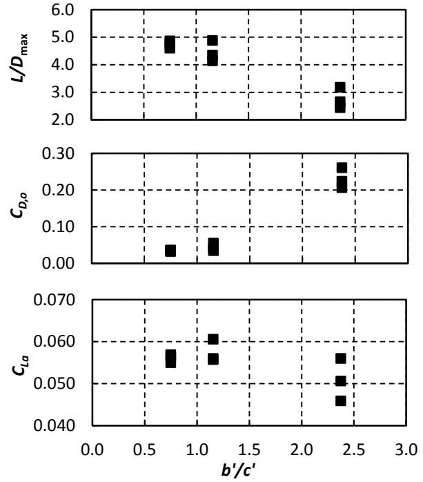
Figure 37. L/D_{max} , C_{D,0} and C_{L,\alpha} vs b'/c'
