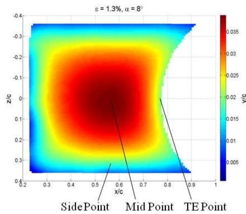
Figure 57. Indication of mid, side, and TE points on 1.3ε wing mean displacement plot: \alpha = 8^\circ
