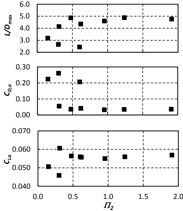
Figure 36. L/D_{max} , C_{D,0} and C_{L,\alpha} vs \Pi_2
