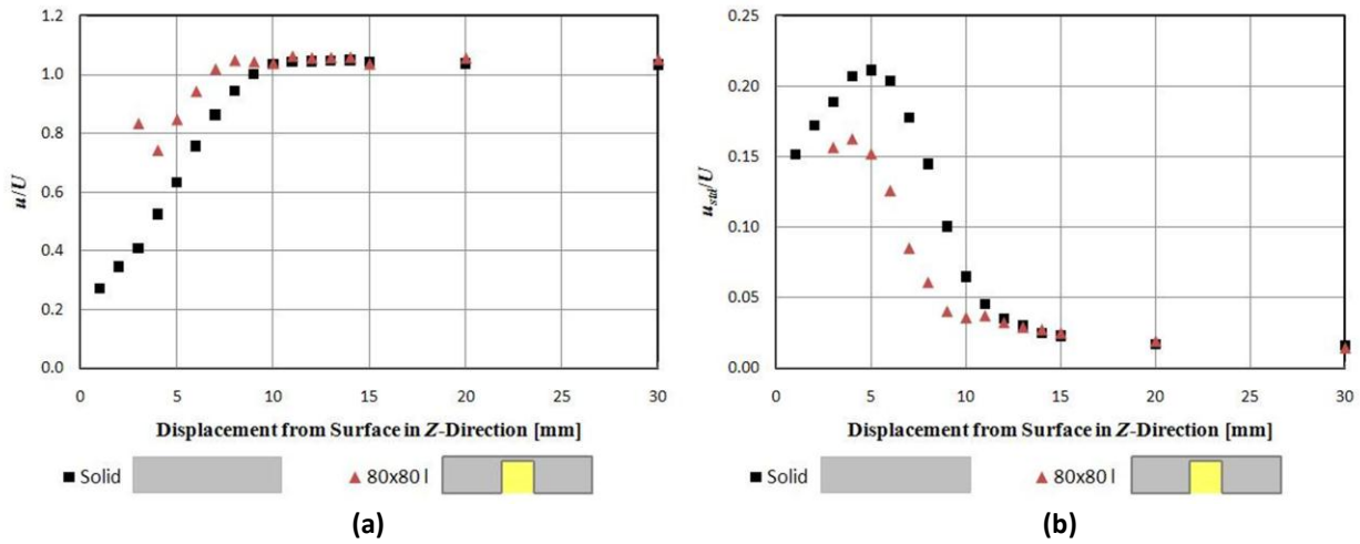
Figure 15. Shear layer size comparison between solid plate and 80x80 latex membrane at 8^\circ angle-of-attack: (a) relative mean velocity magnitude, (b) relative velocity standard deviation
