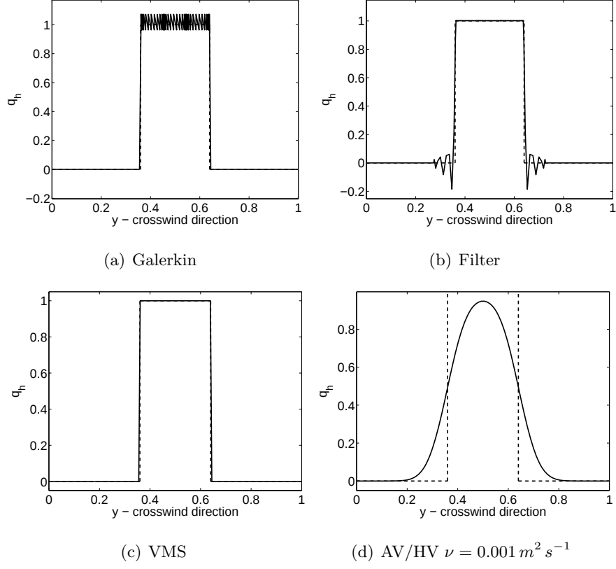
Figure 23: Tr2-2D : Crosswind cut at 0.5 m in the x-direction. \Delta t = 0.001 \text{ s} , 11 \times 11 elements with 11^{th} order polynomials. Results at t = 2 \text{ s} (after 1 periodic revolution along x). Solid line indicates the computed solution. The dashed line is the analytic solution.
