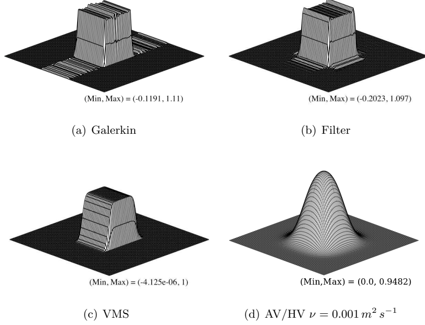
Figure 21: Tr2-2D : Surface plot of the concentration field: \Delta t = 0.001 \text{ s} (except for HV: \Delta t = 0.0002 \text{ s} ), 11 \times 11 elements with 11^{th} order polynomials. Results at t = 2.0 \text{ s} (after 1 periodic revolution along x ).
