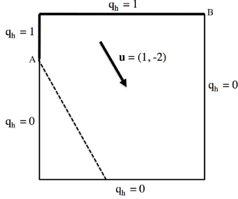
Figure 7: St-2D : initial configuration of the steady-state problem
