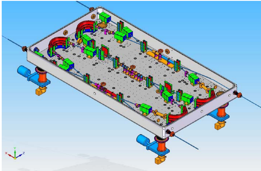
Figure 3: A technical schematic of the heart of the DESIREE facility: the double-walled vacuum vessel, showing the open ion optics, the two separate storage rings, and the unique merging region.
