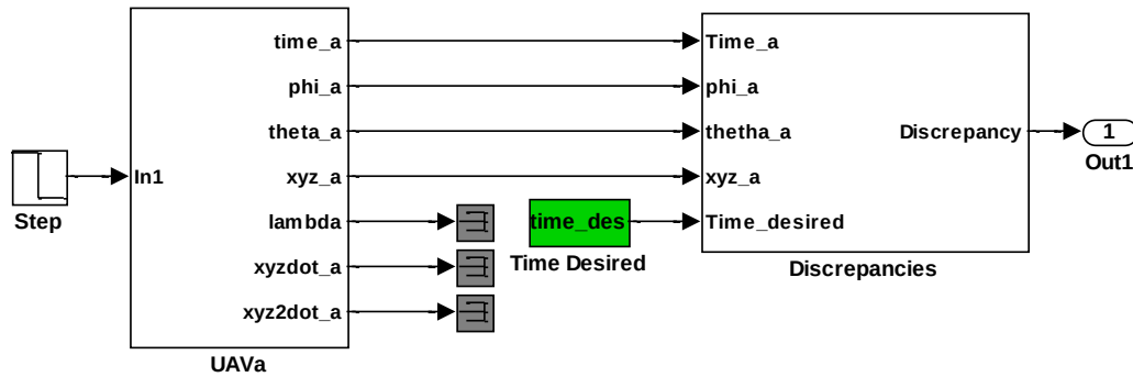
Figure 65: Overview of the Optimal Trajectory Generator.
