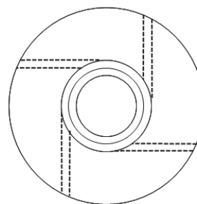
4 tangential inlets
